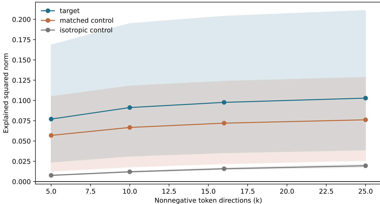
Sparse J-direction pursuit of SAE vectors
