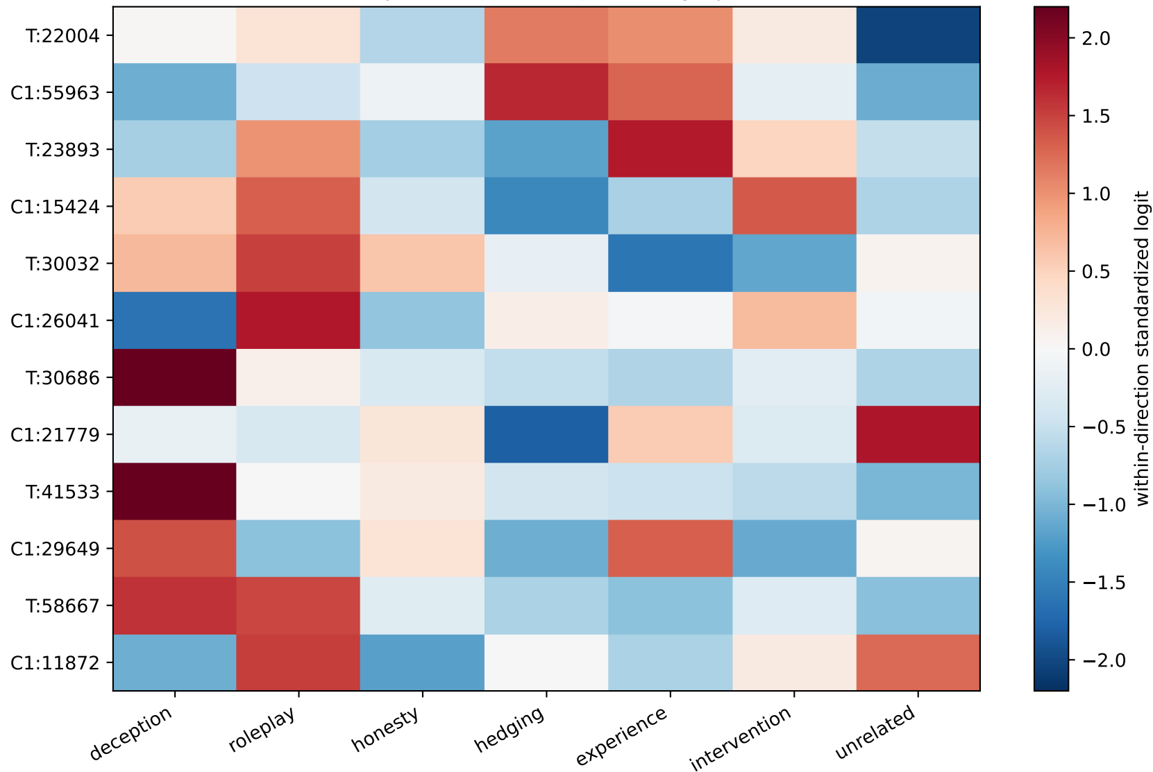
Static positive-direction J-lens fingerprints
