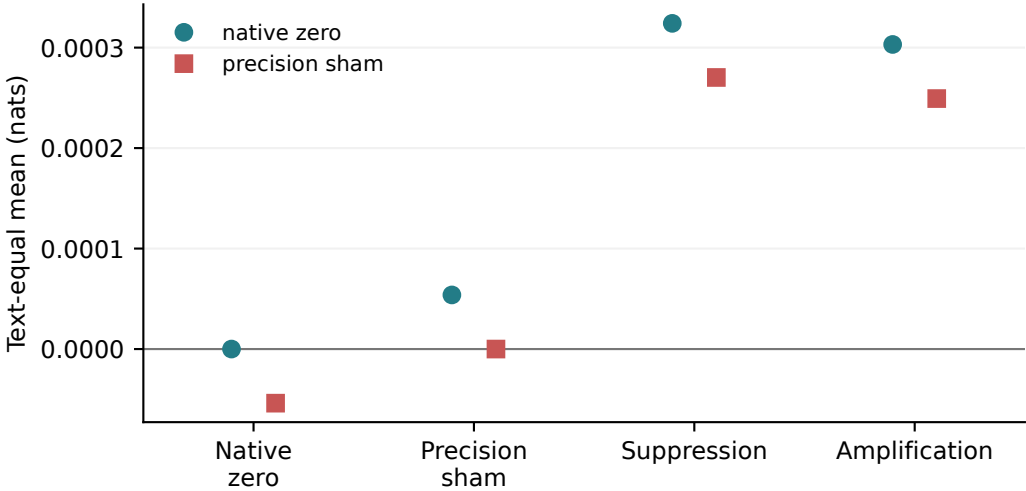
Paired NLL difference: mode minus reference
