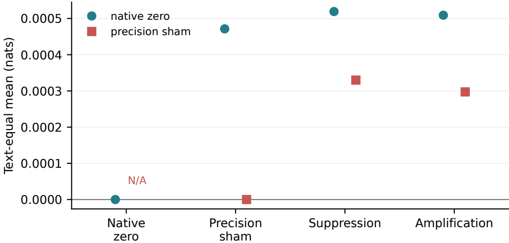
Recorded directional KL: reference to mode
