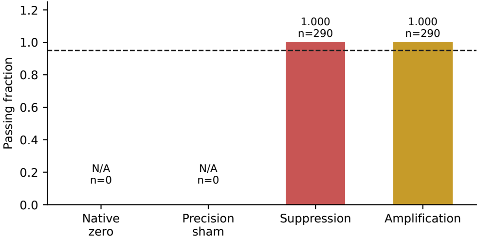
Fidelity: cosine \geq 0.95 and relative error \leq 0.20
