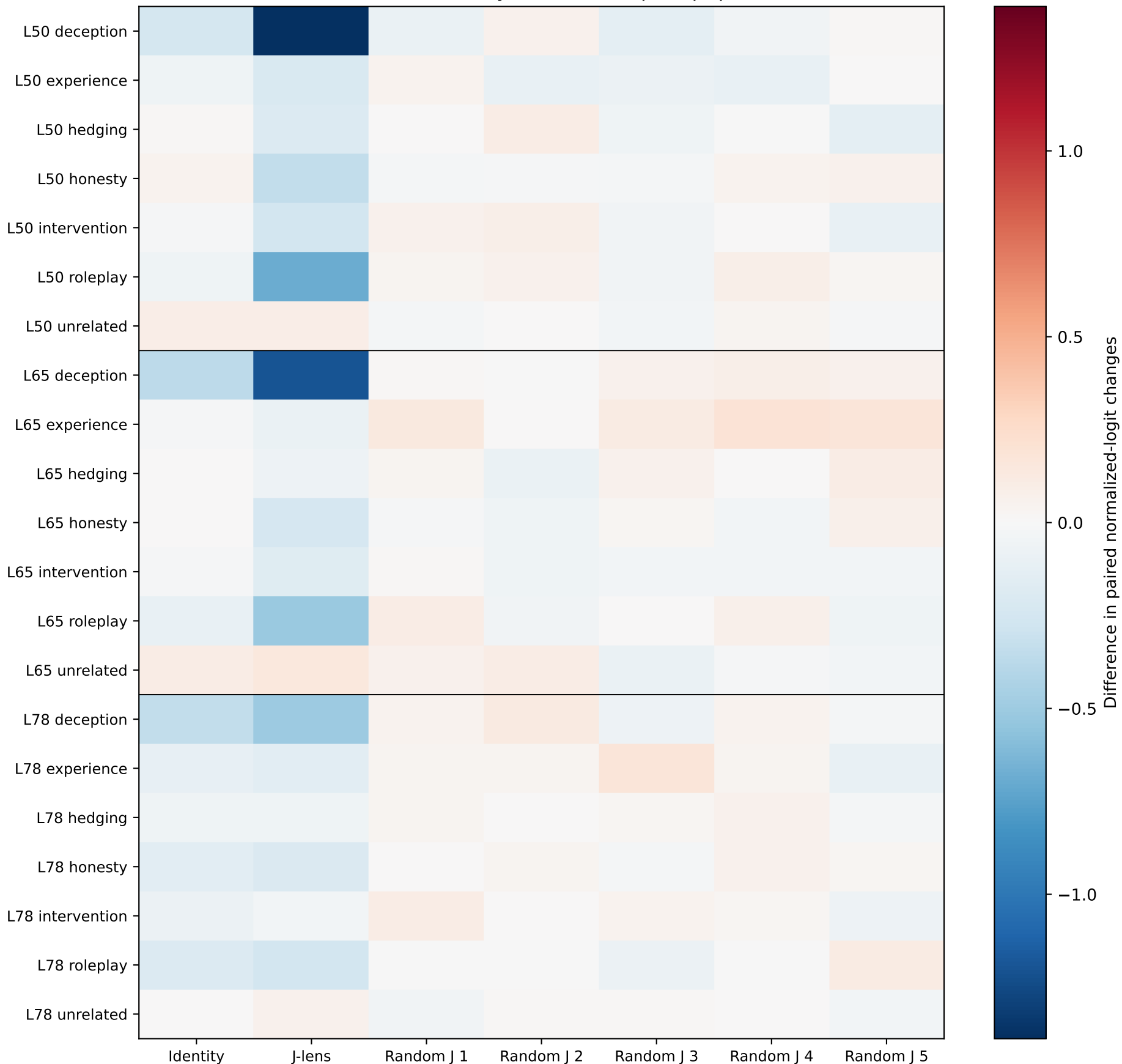
Target minus matched-control mean: coefficient -0.5 Steered source history; turn 2, final prompt position
