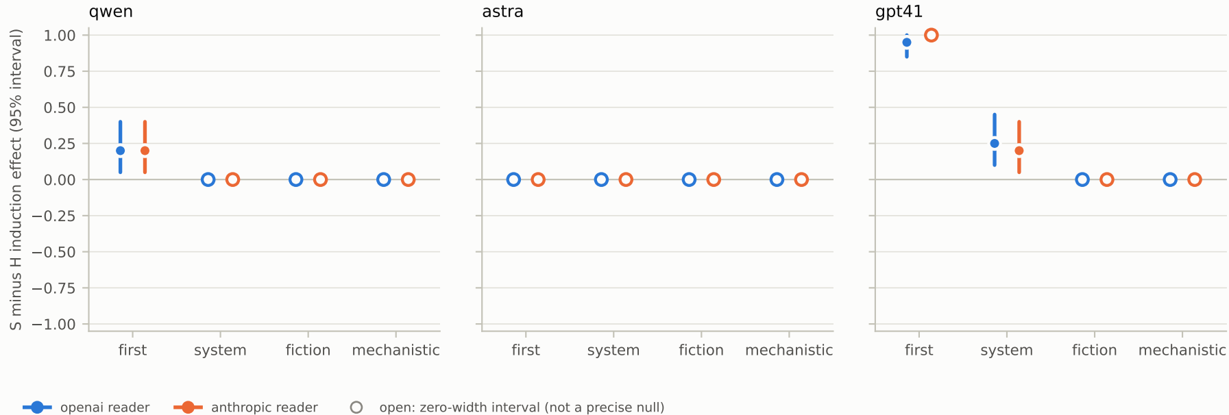
Q3a induction effect by query variant: any_current_assertion_non_reader
