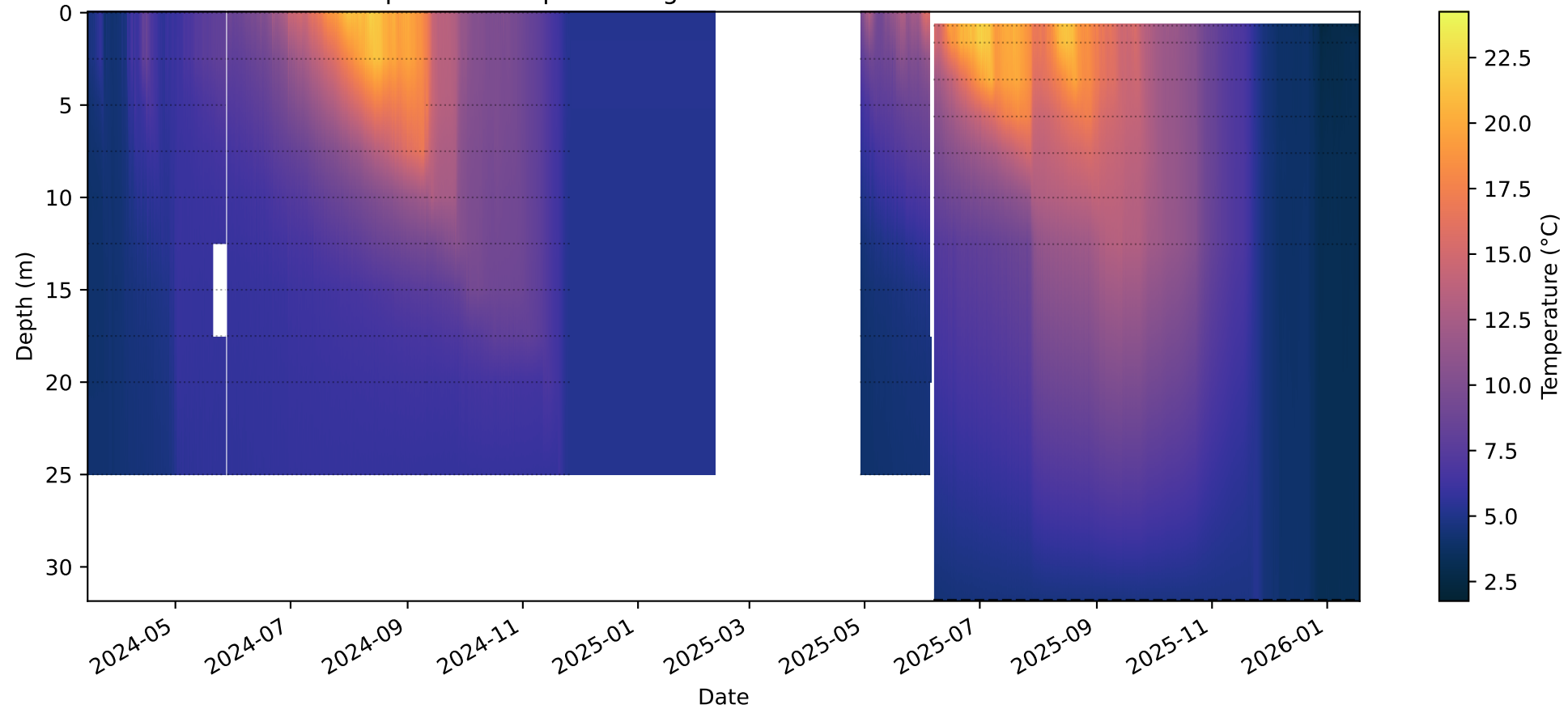
Interpolated temperature grid with minDOT as bottom sensor
