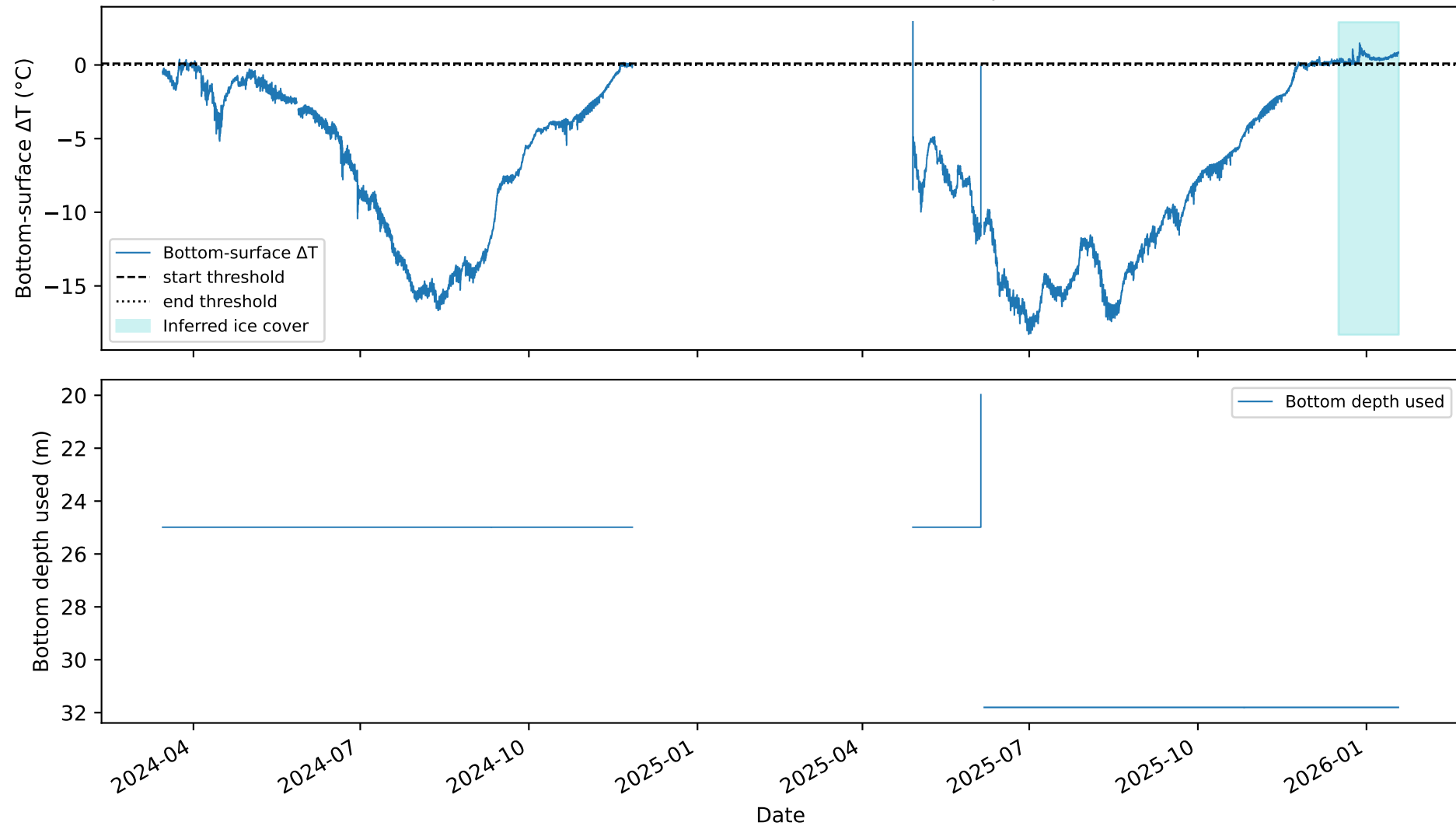
Ice cover: start \Delta T \geq 0.10 °C, end \Delta T \leq 0.00 °C | miniDOT: yes
