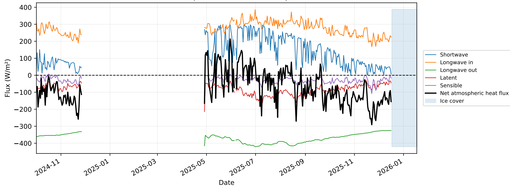
Surface heat-flux components and net atmospheric heat flux
