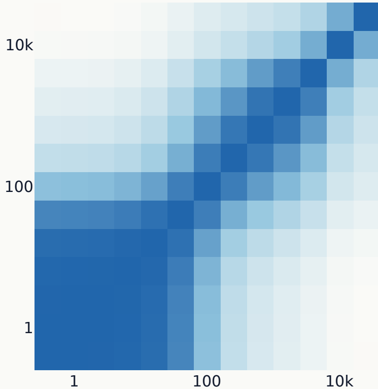
Grid (train) · logits
