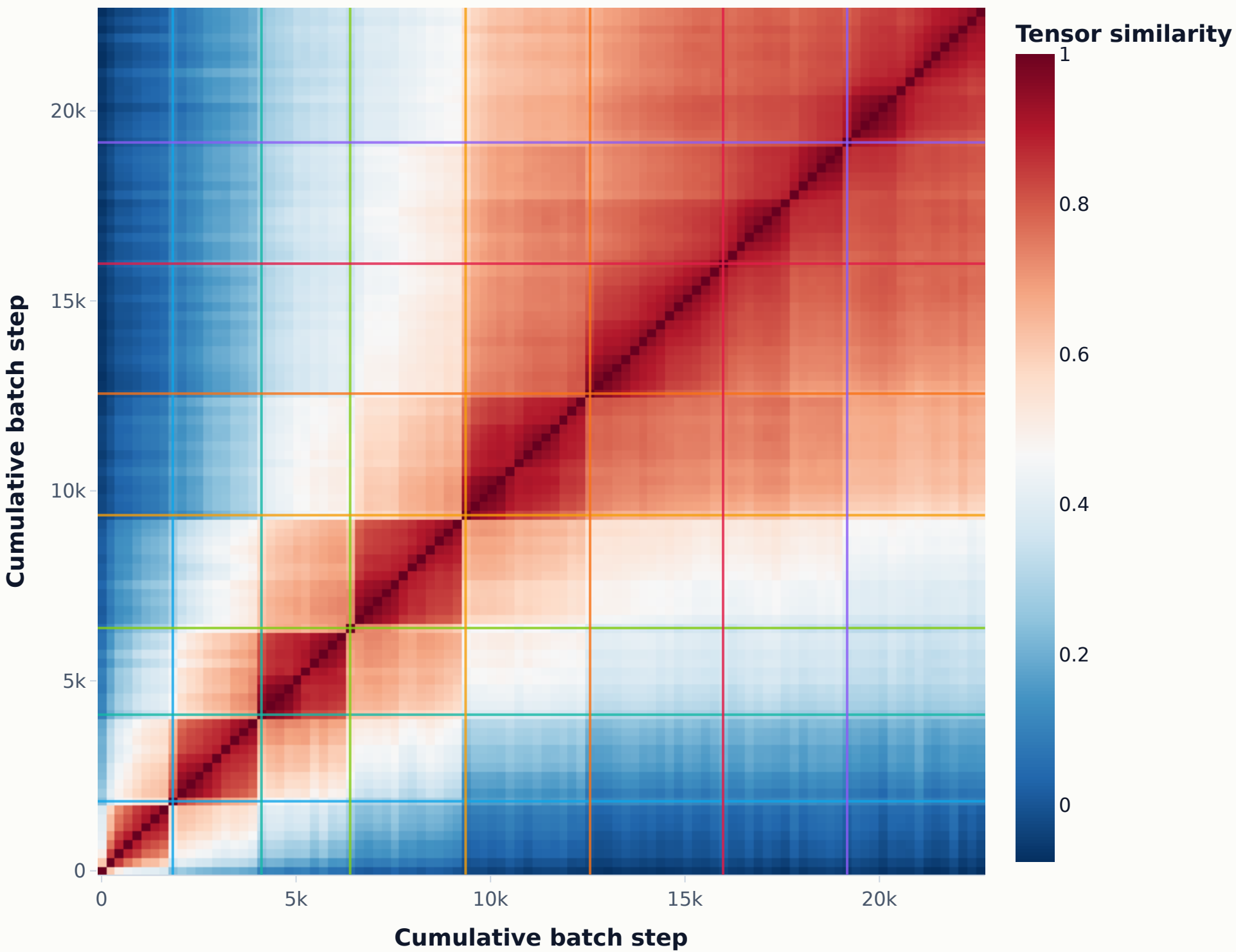
Curriculum shift checkpoint heatmap
