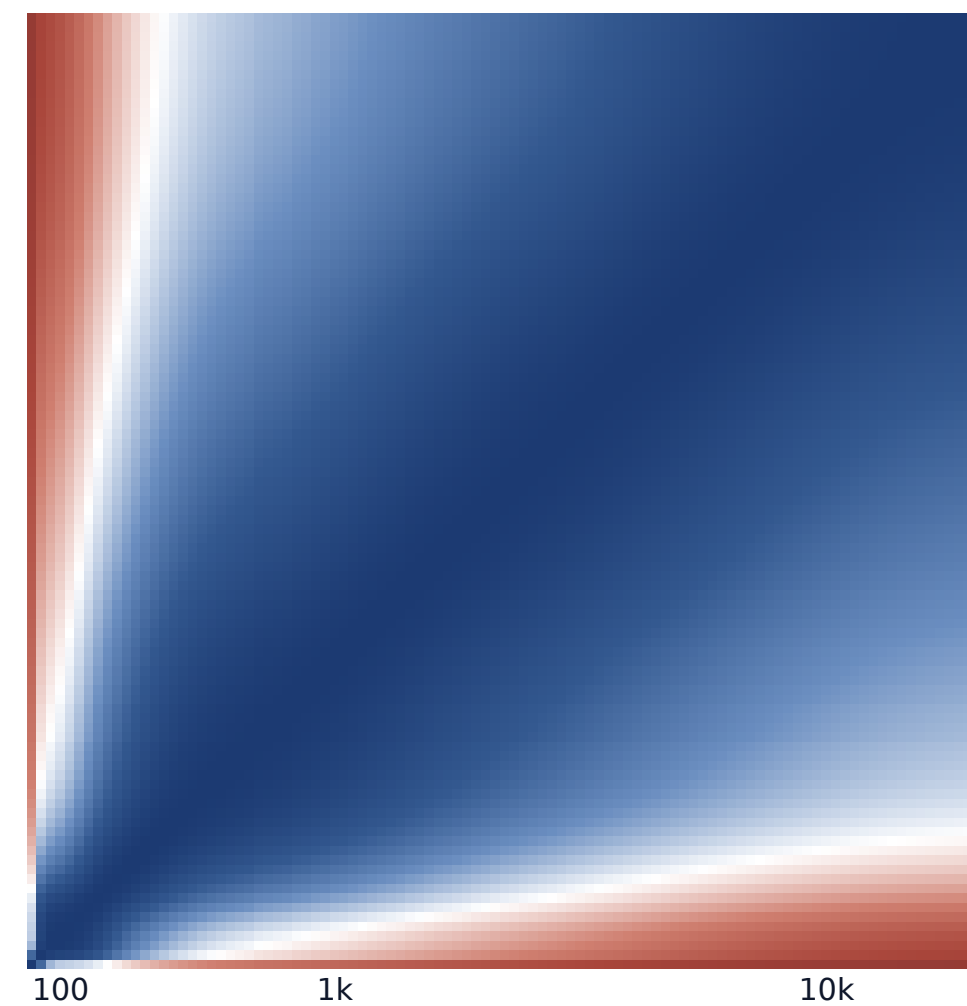
Matrix cosine
