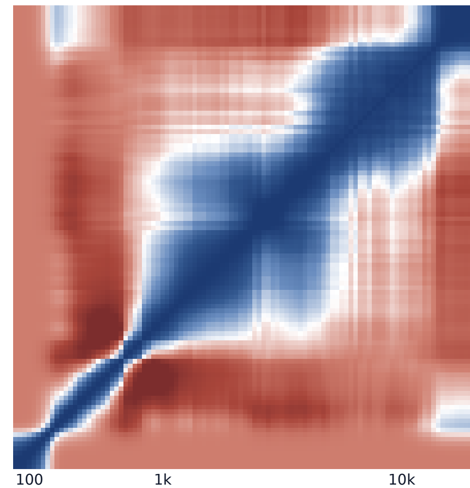
Matrix cosine
