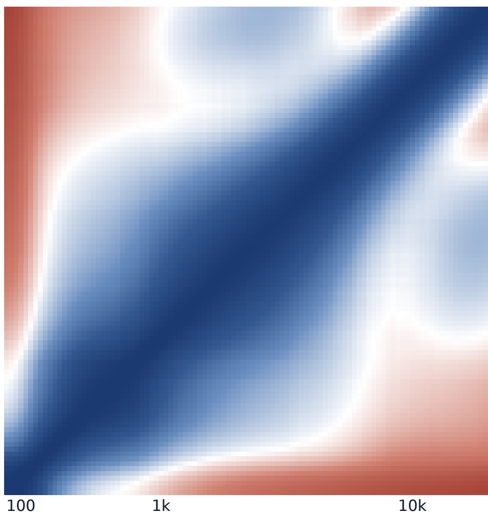
Pile · residual
