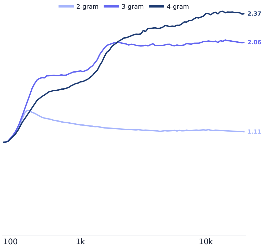
Pile · residual
