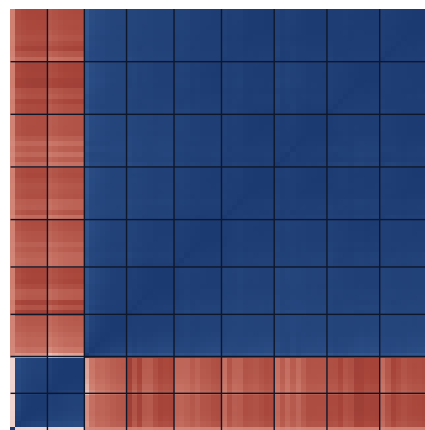
class 6
