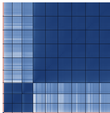
class 7
