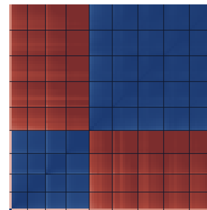
class 8
