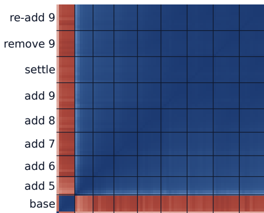
class 5
