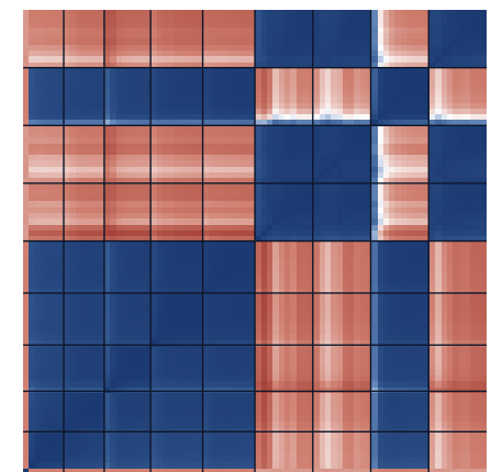
class 9
