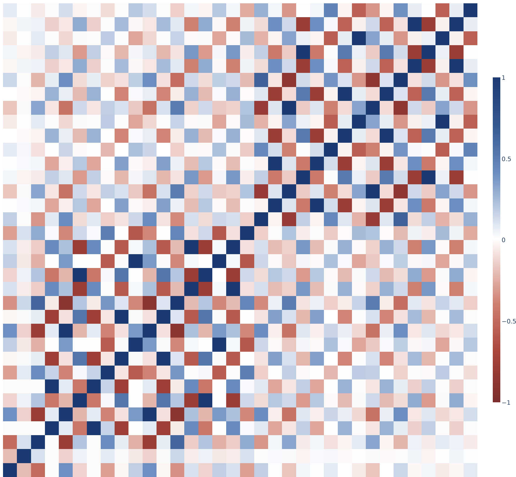
Path-pair tensor similarity · step 6000, 34 paths (direct, layer1, 32 layer2 paths)
