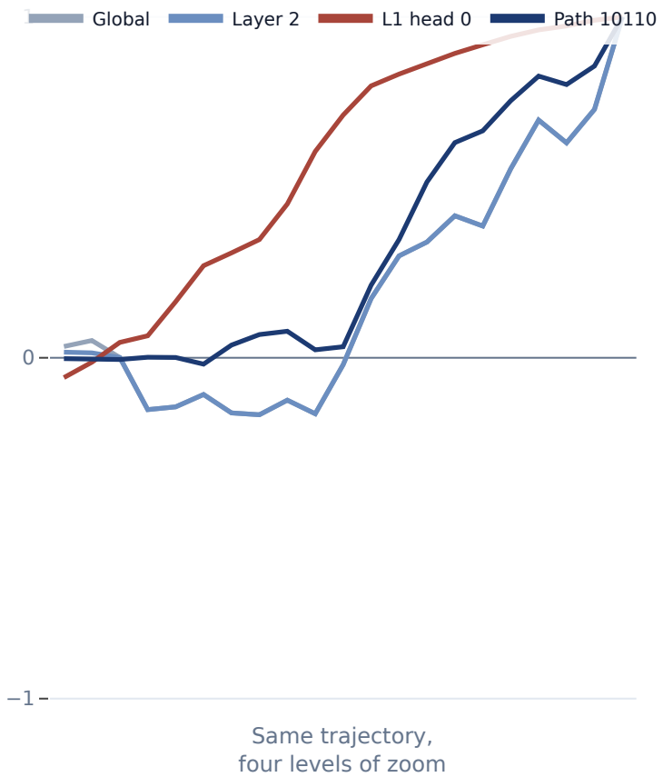
Similarity to final · per decomposition
