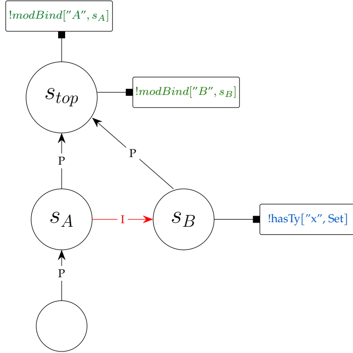
Figure 4.2: Resulting scope graph of 4.6.3
