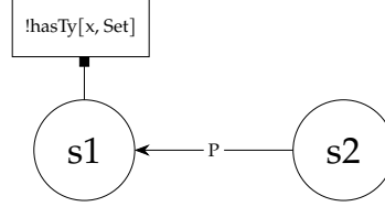
Figure 4.1: Scope graph of listing 4.2
