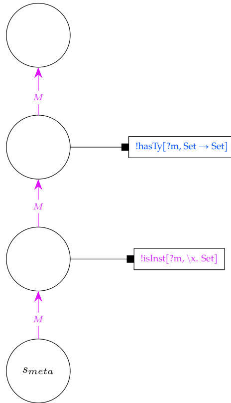
Figure 5.1: Example scope graph with metavariables
