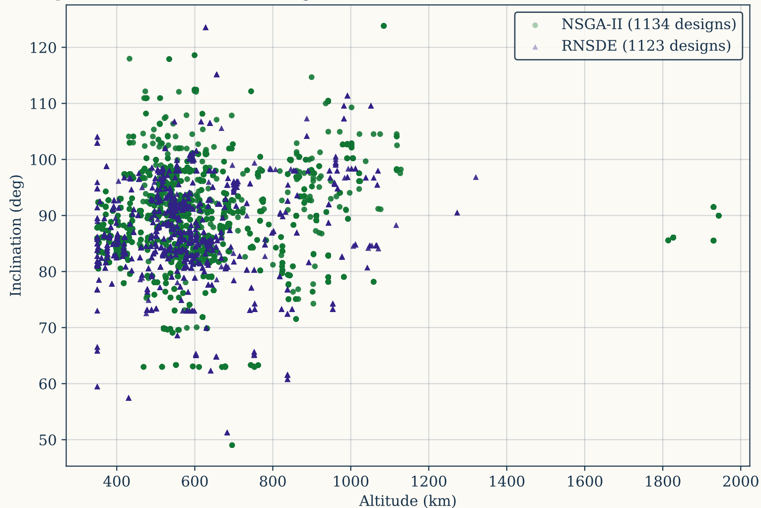
Part-B siting of the two candidates: orbital slots of promising designs (pooled strict front-0, CVaR-90 g1000 matrix, 4 families x 16 seeds, 69472 satellite slots)
