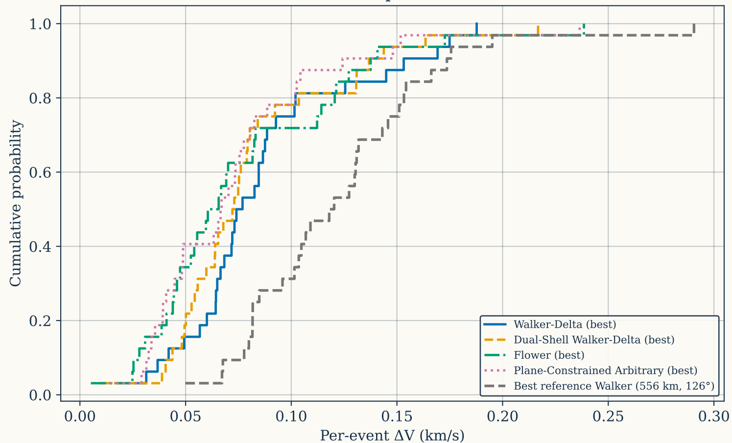
Per-event \Delta V distribution: optimized vs reference Walker
