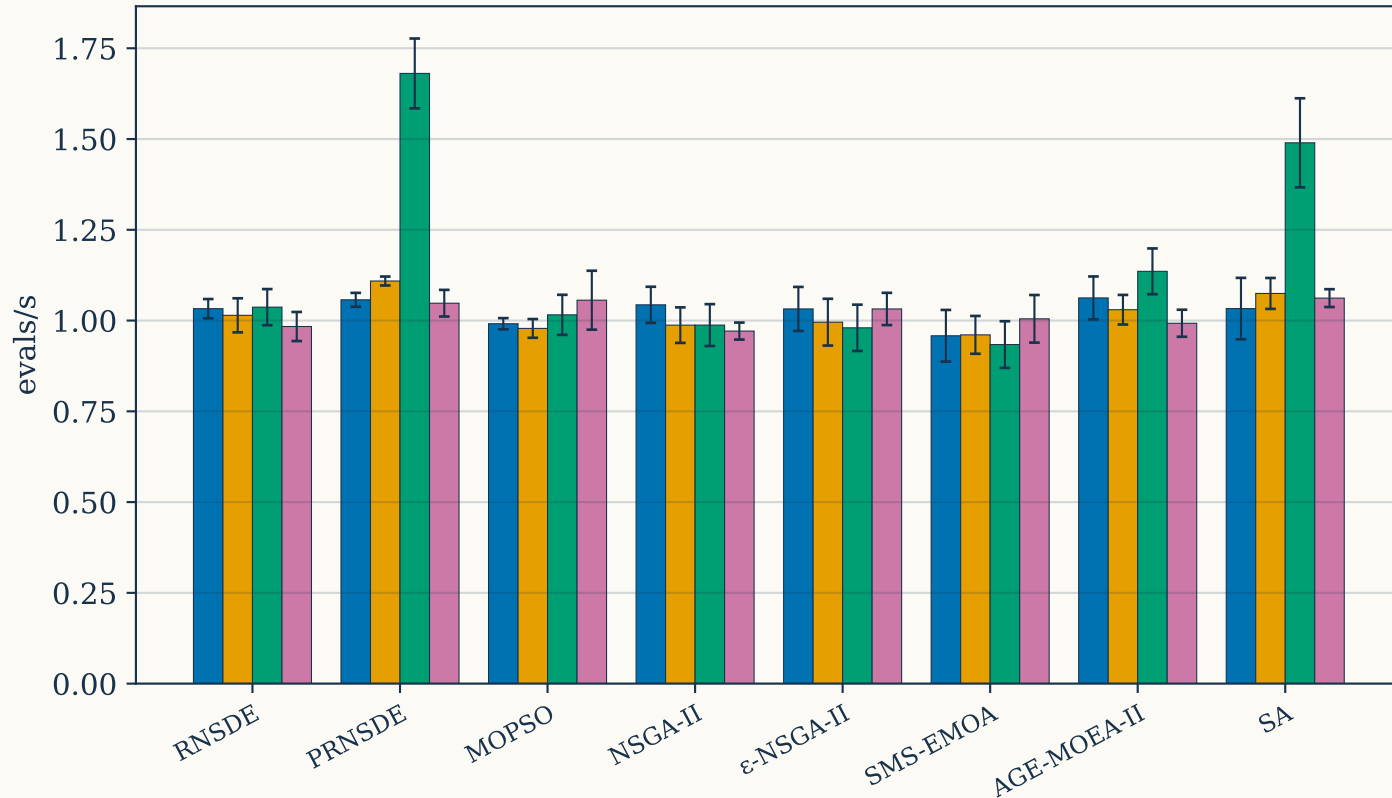
Objective evals / s (▲ better; sms_emoa single-stream)
