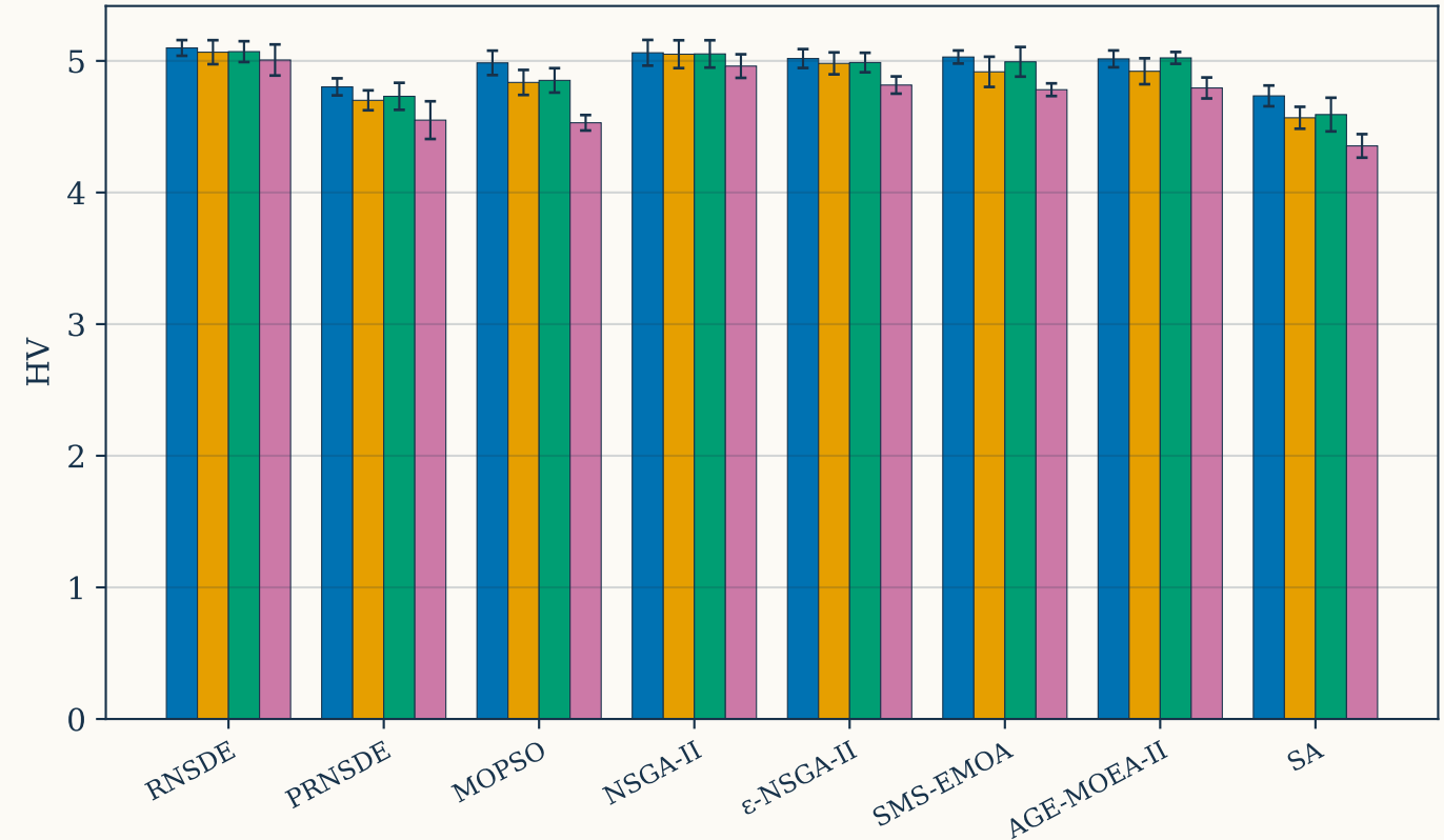
Mean hypervolume (▲ better, log space)
