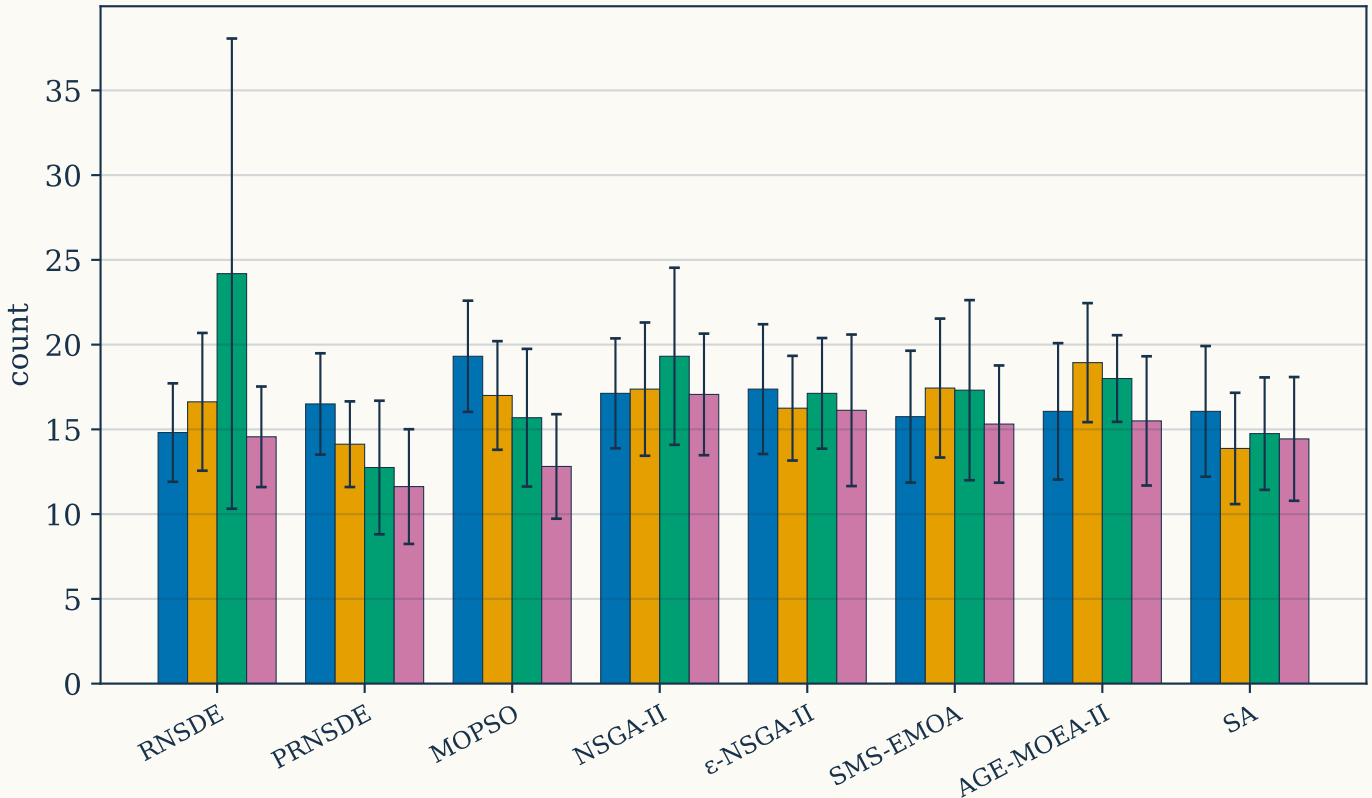
Pareto front size (▲ better)
