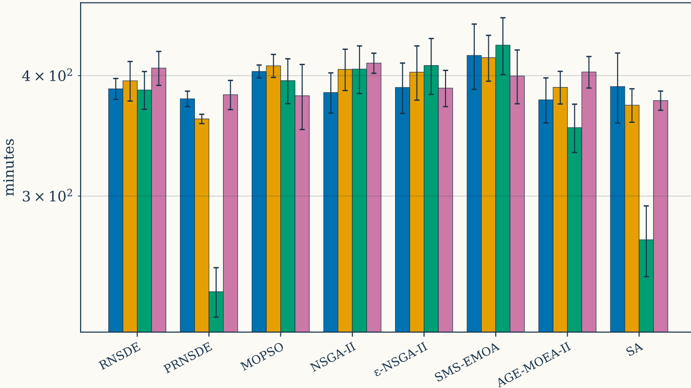
Optimize wall time (▼ better, log; sms_emoa single-stream)
