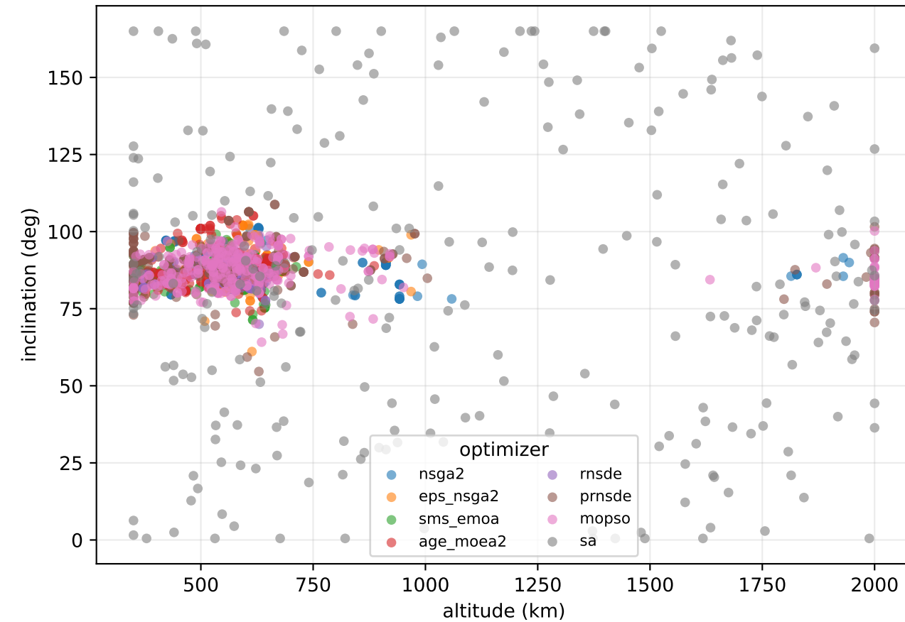
All walker Pareto designs (n=2128)
