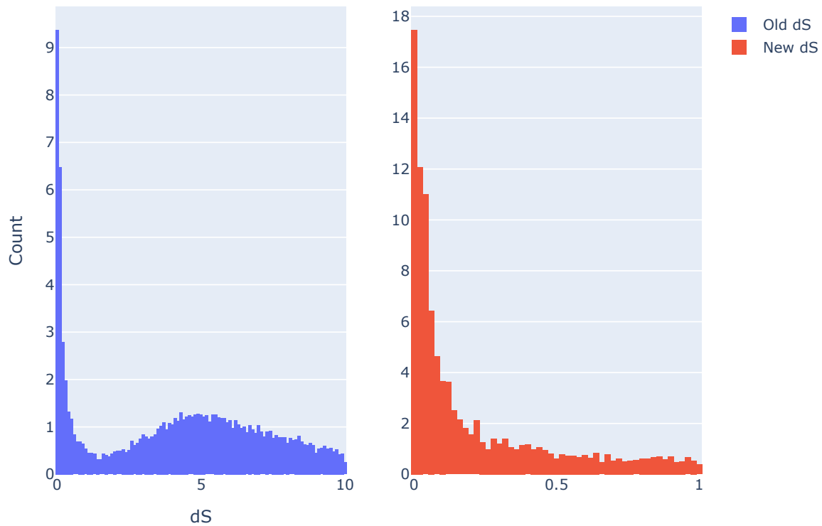
Distribution of old vs. new dS values ( D. discoideum )
