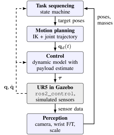
Fig. 1. Control pipeline. Solid arrows show the forward flow of commands and data between stages; dashed arrows show joint-state feedback from the robot.
