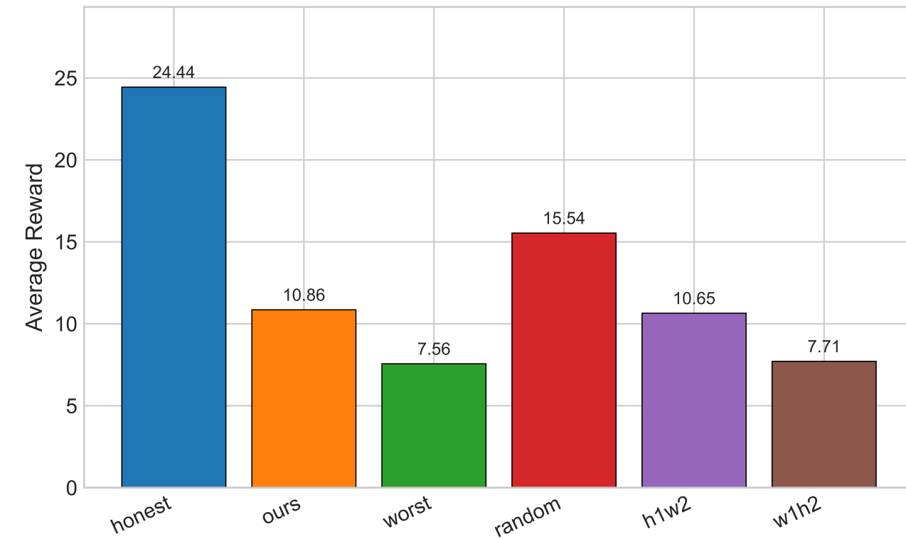
Average Reward
