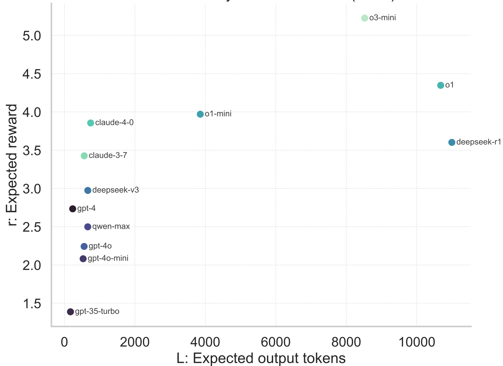
Model Efficiency–Reward Frontier (L vs r)
