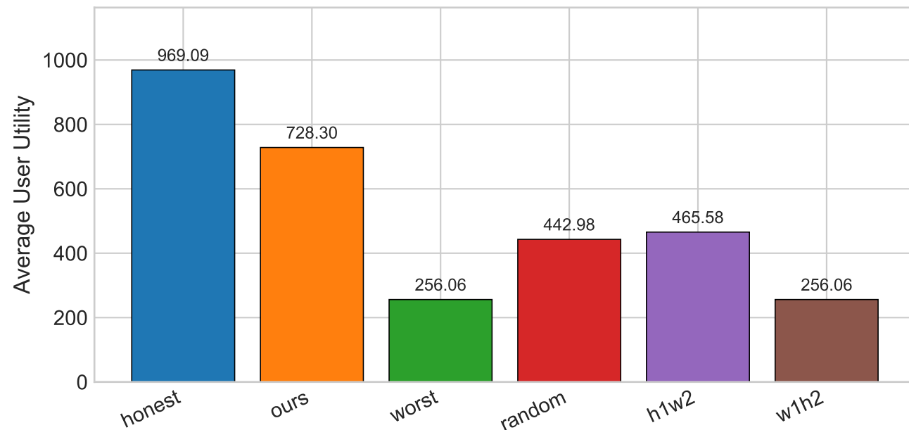
Average User Utility
