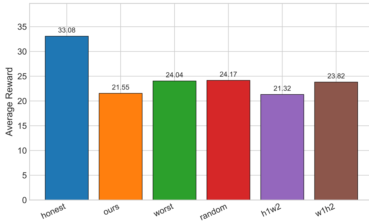
Average Reward
