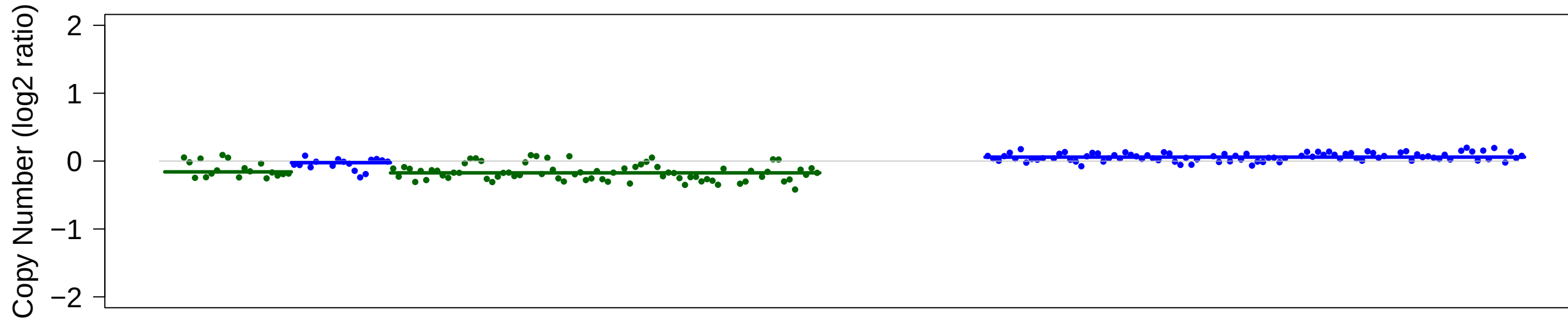
Chromosome chr1
