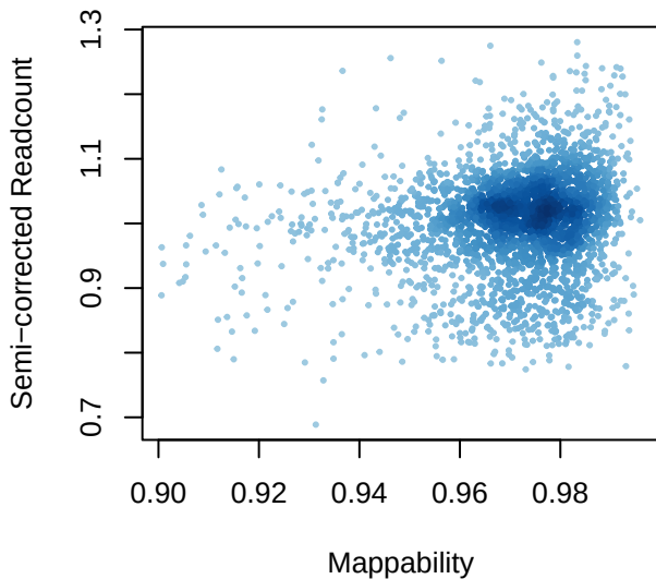
Mappability Bias in GC-Corrected Readcounts
