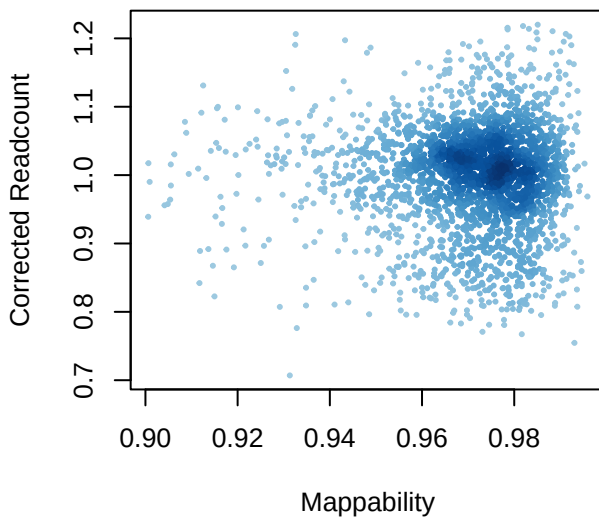
GC and Mappability Corrected Readcounts
