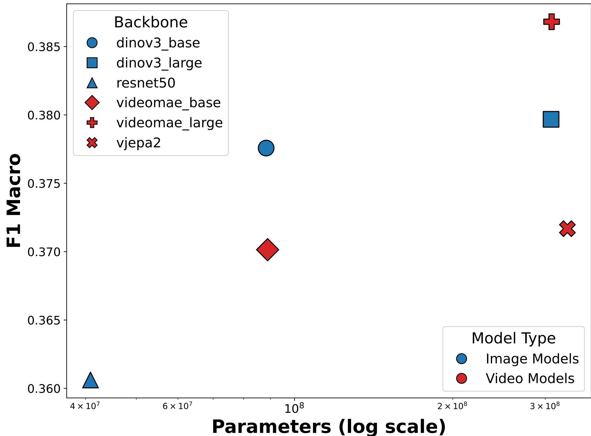
Performance vs Model Size (Attention)
