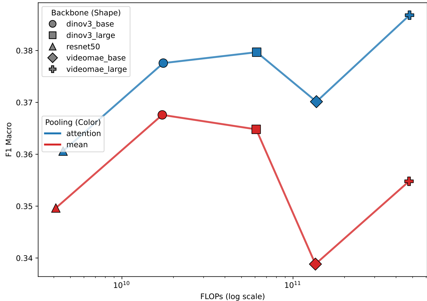
Performance vs Compute
