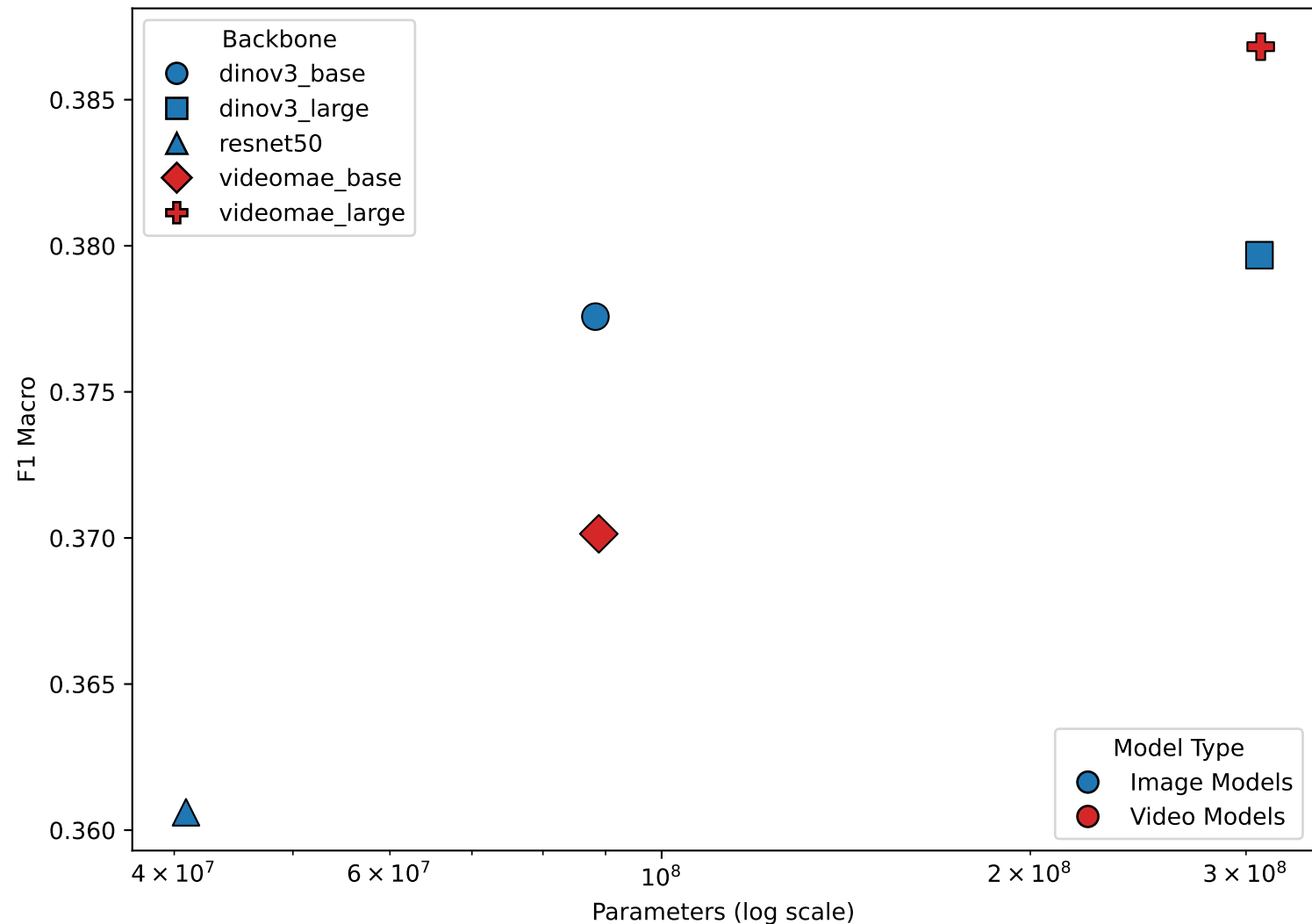
Performance vs Model Size (attention)
