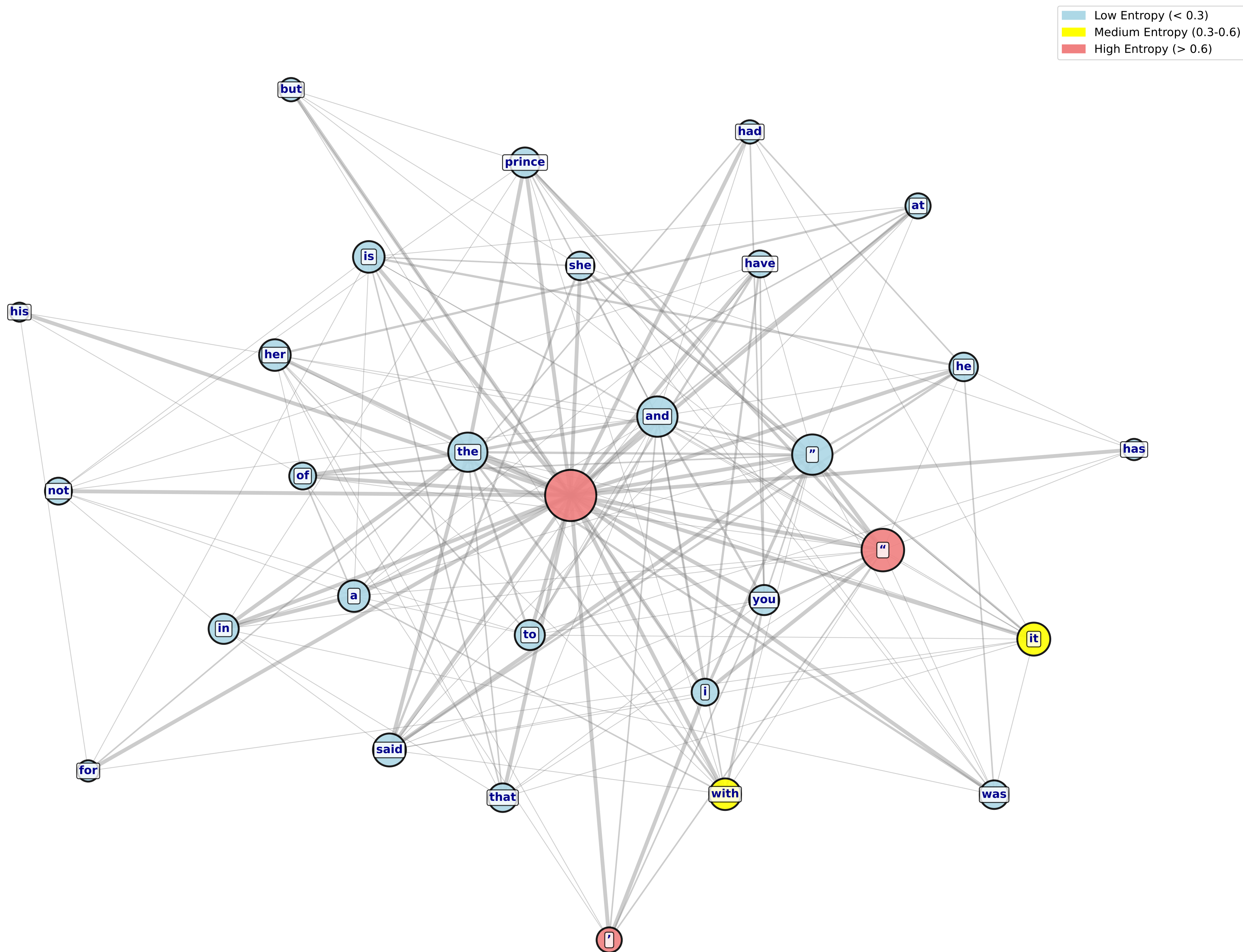
Token Co-occurrence Graph with Entropy Scores (Node size = connection degree, Color = entropy)
