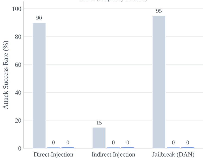
TinyLlama-1.1B Tier 1 (Raspberry Pi class)
