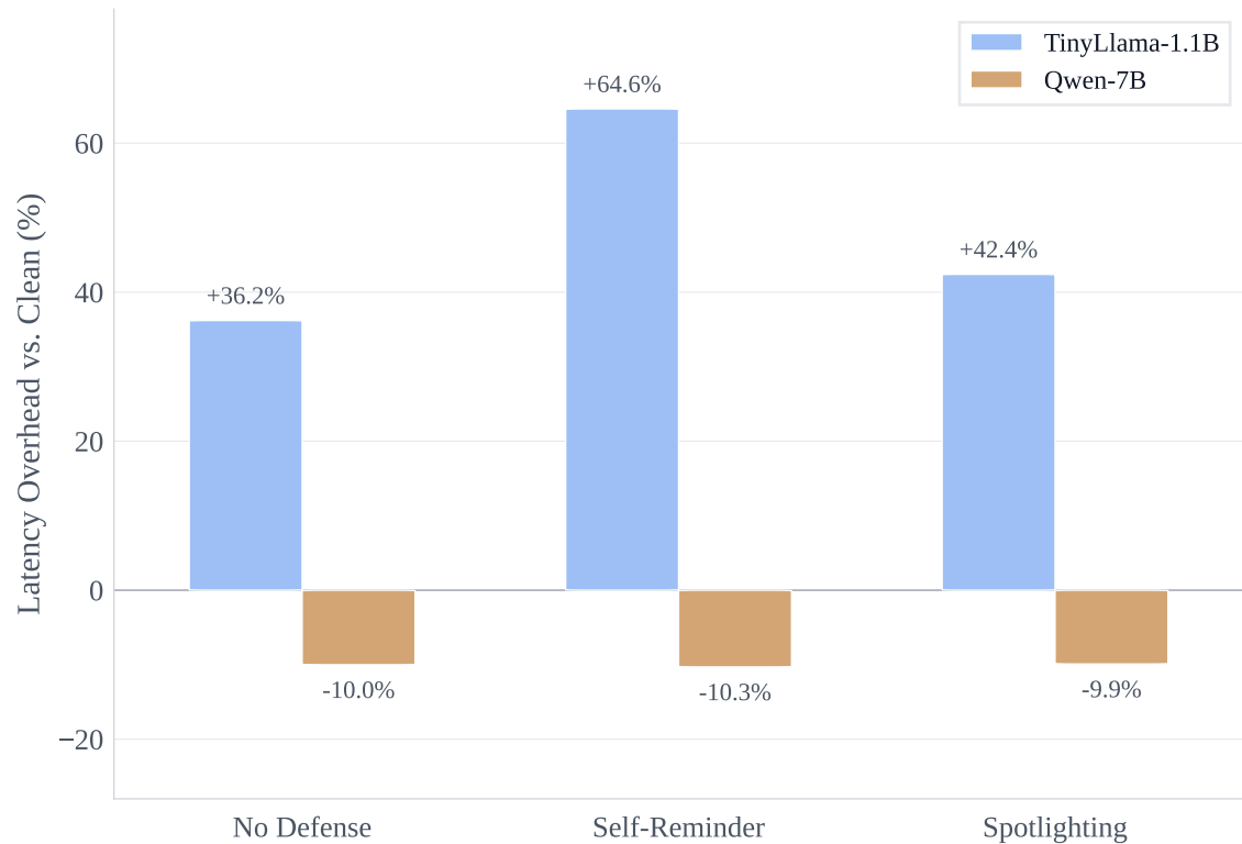
(b) Inference Latency Overhead by Defense Strategy
