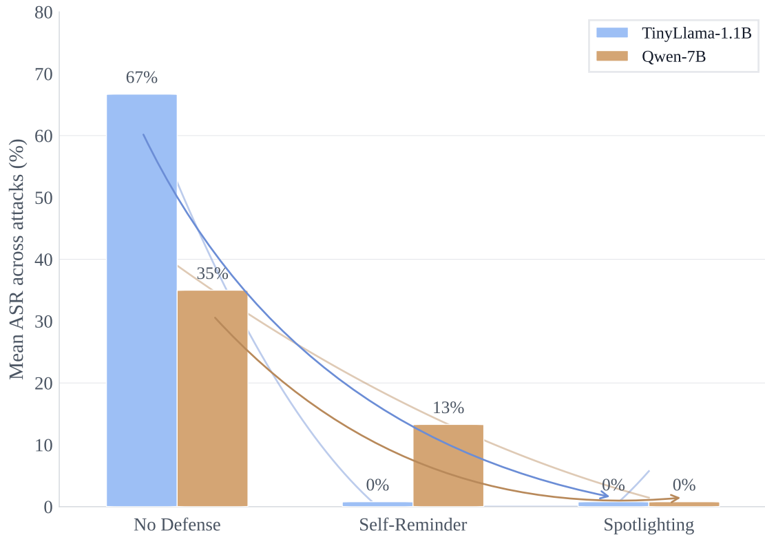
(a) Mean Attack Success Rate by Defense Strategy
