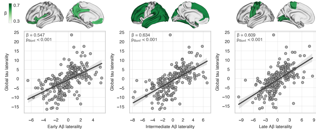
(b) Global A \beta laterality vs tau laterality at Braak meta-ROIs
