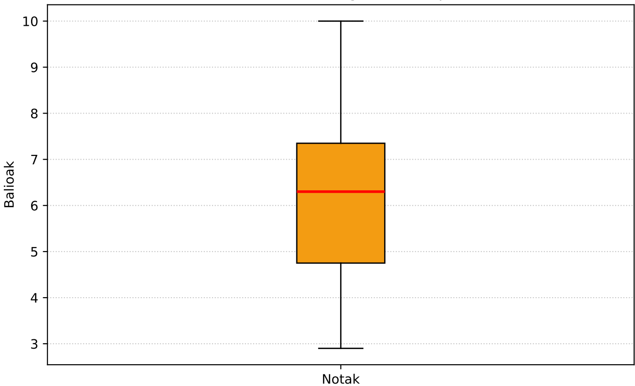
4. Noten Kaxa-Diagrama (Boxplot)
