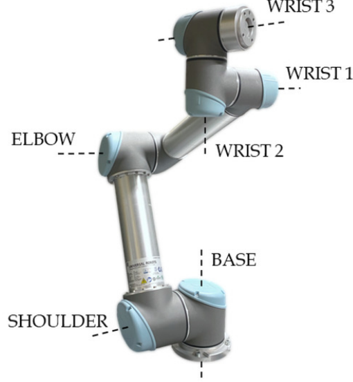
Figure 6: Labeled structure of the UR3 robotic arm, showing the six rotational joints: Base, Shoulder, Elbow, Wrist 1, Wrist 2, and Wrist 3. [2]
