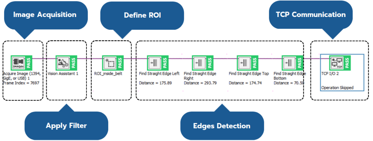
Figure 2: NI Vision Builder pipeline for box detection
