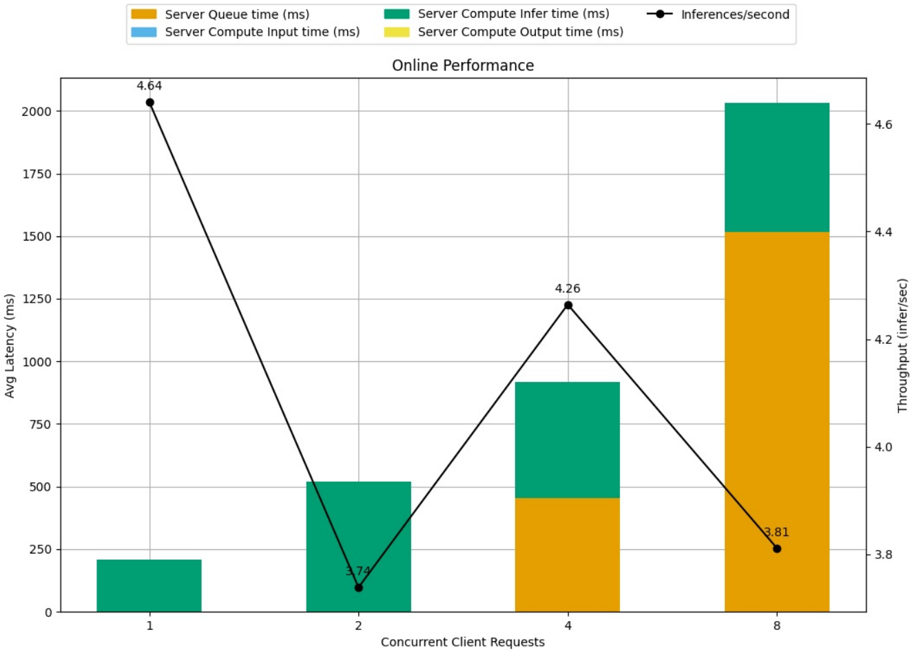
Latency Breakdown for Online Performance of yolov8s_config_0
