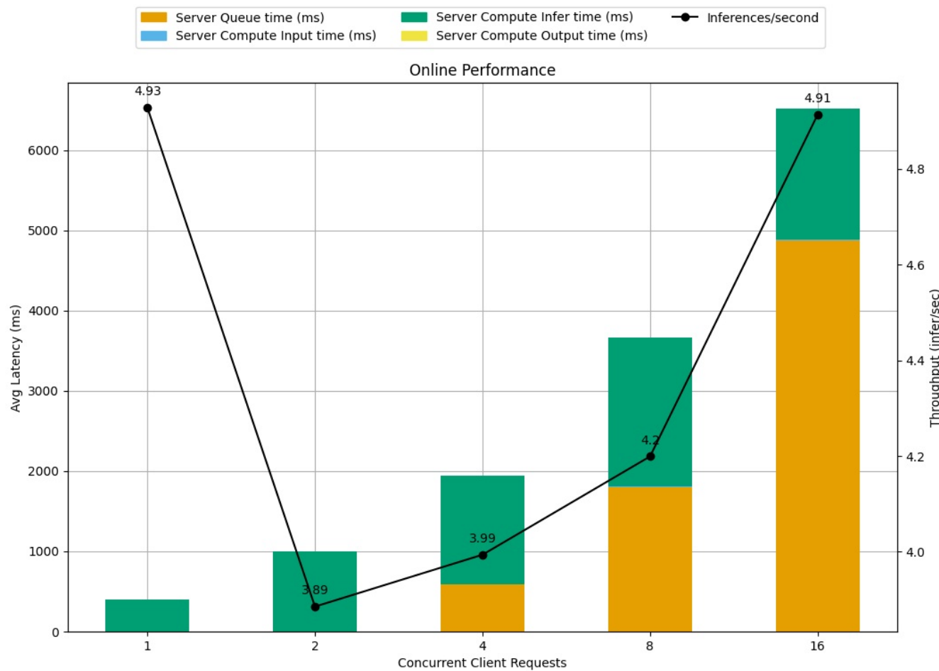
Latency Breakdown for Online Performance of yolov8s_config_15
