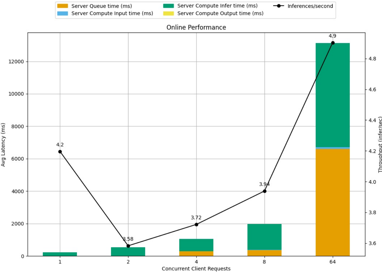
Latency Breakdown for Online Performance of yolov8s_config_6
