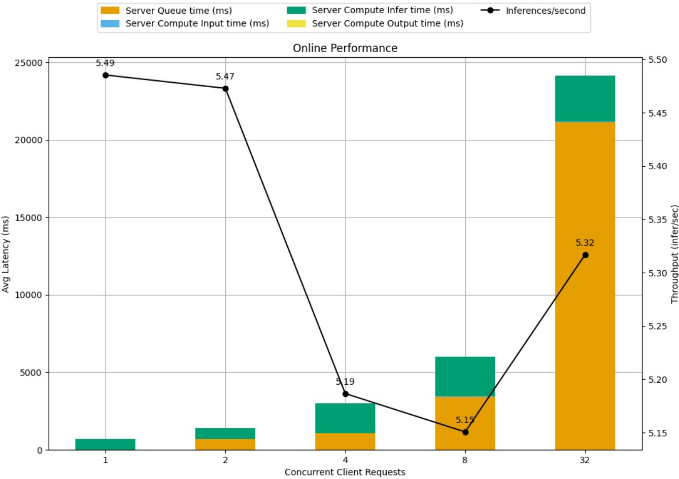
Latency Breakdown for Online Performance of yolov8s_config_7
