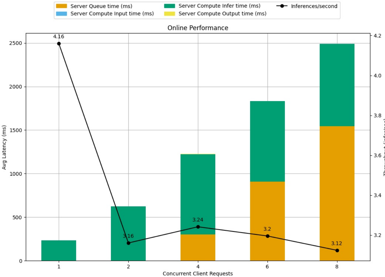
Latency Breakdown for Online Performance of yolov8s_config_10
