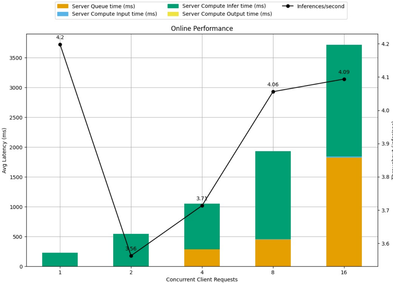
Latency Breakdown for Online Performance of yolov8s_config_5
