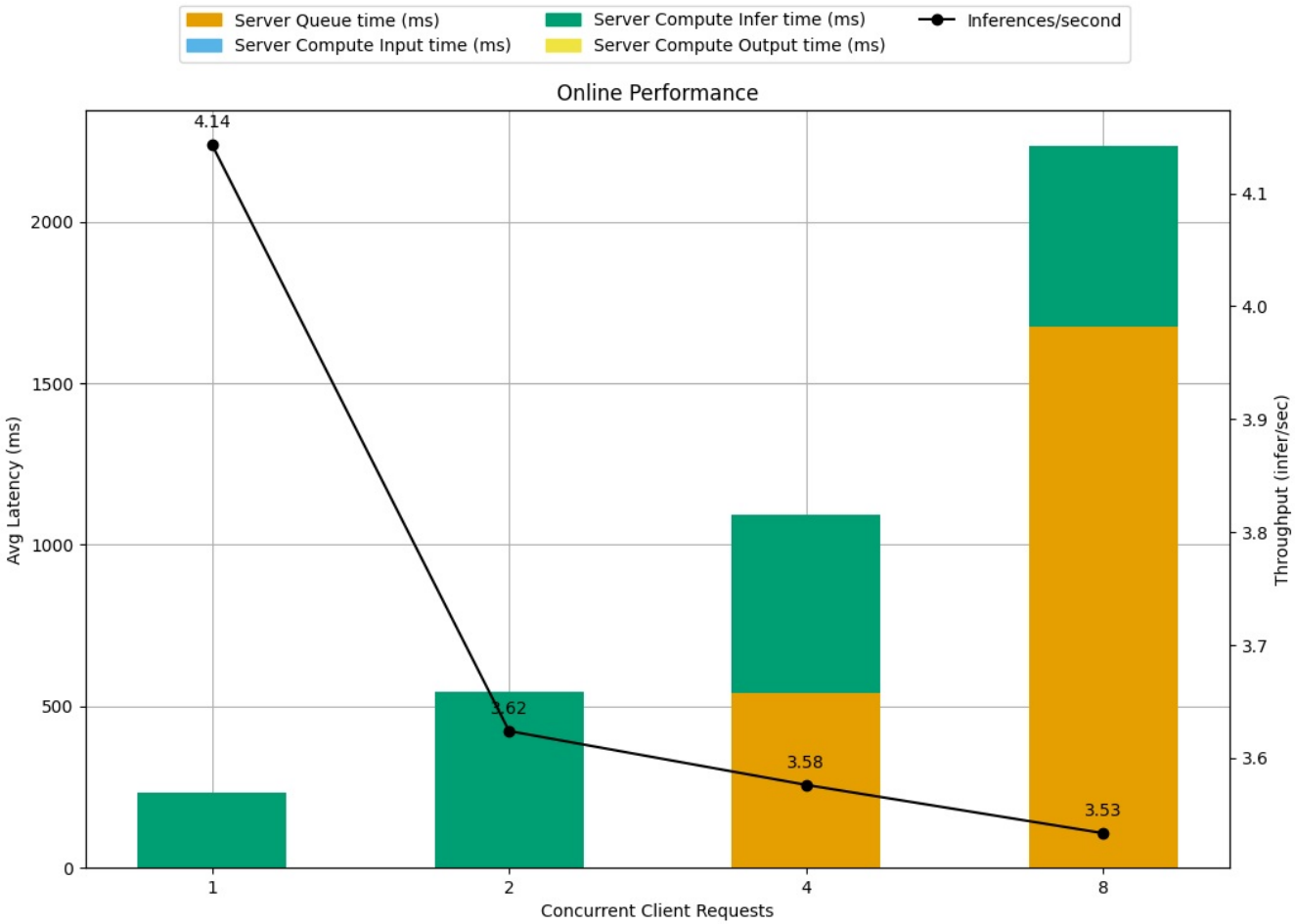
Latency Breakdown for Online Performance of yolov8s_config_8
