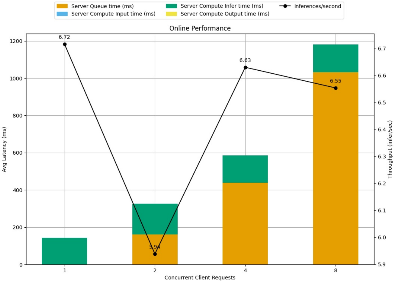
Latency Breakdown for Online Performance of yolov8s_config_11
