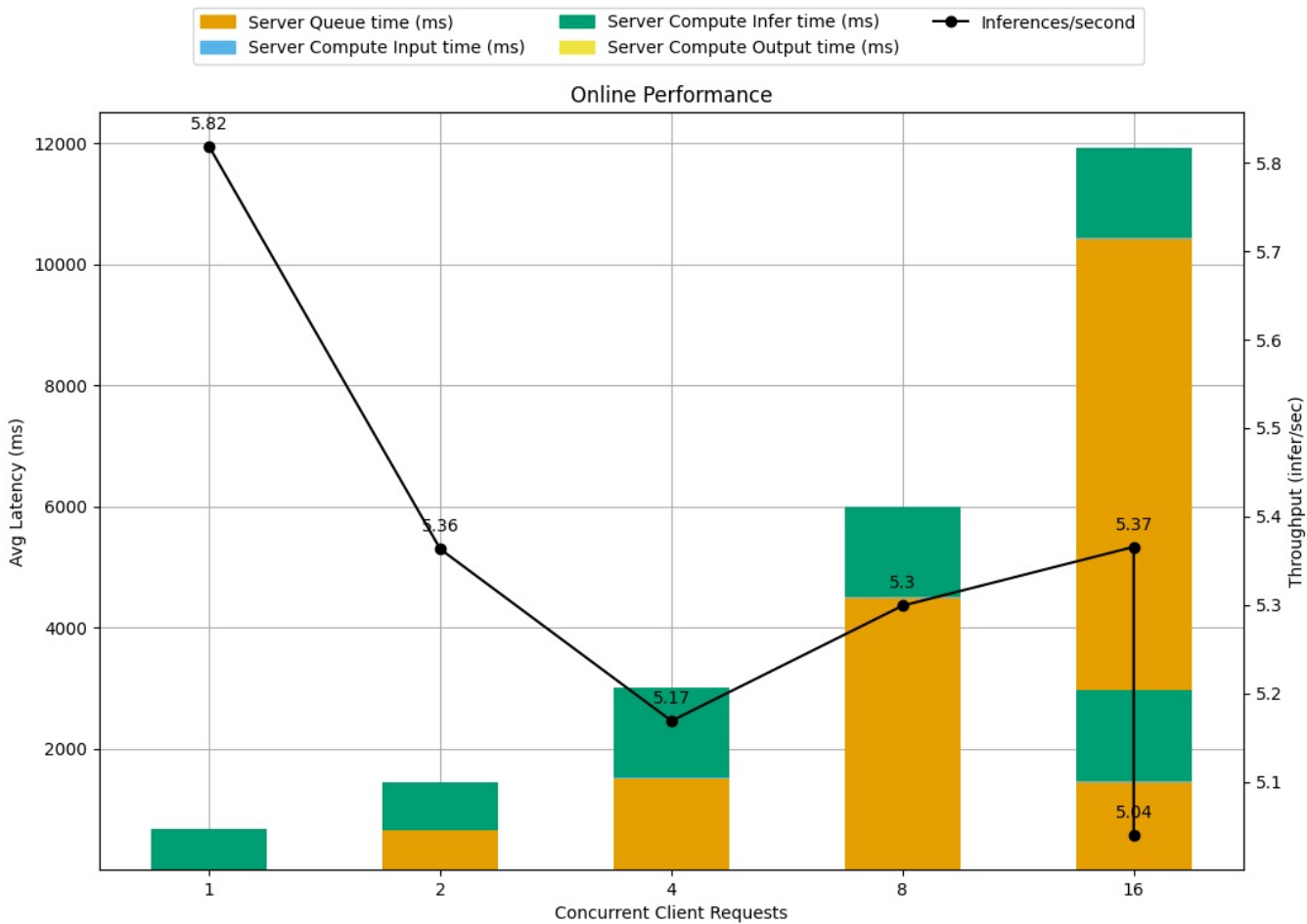
Latency Breakdown for Online Performance of yolov8s_config_12
