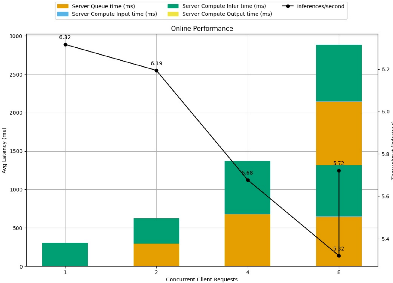
Latency Breakdown for Online Performance of yolov8s_config_13
