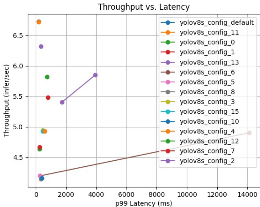
Throughput vs. Latency curves for 15 best configurations.
