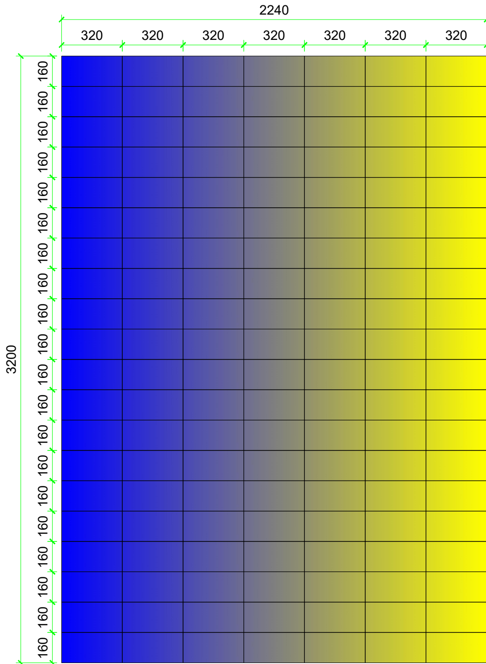
01 LED SCREEN FRONT ELEVATION SCALE 1 : 50
