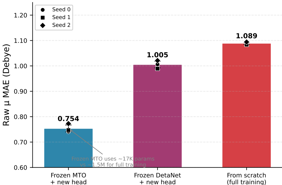
Fig 18 | Frozen-probe representation-reuse experiment (3 seeds, 5k QM9S molecules, 20 epochs). Bars: mean \pm SD across seeds. Points: individual seeds. Lower is better.
