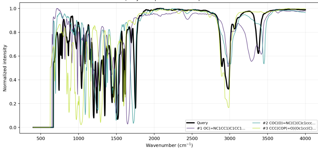
Query vs Top-K Candidate Spectra
