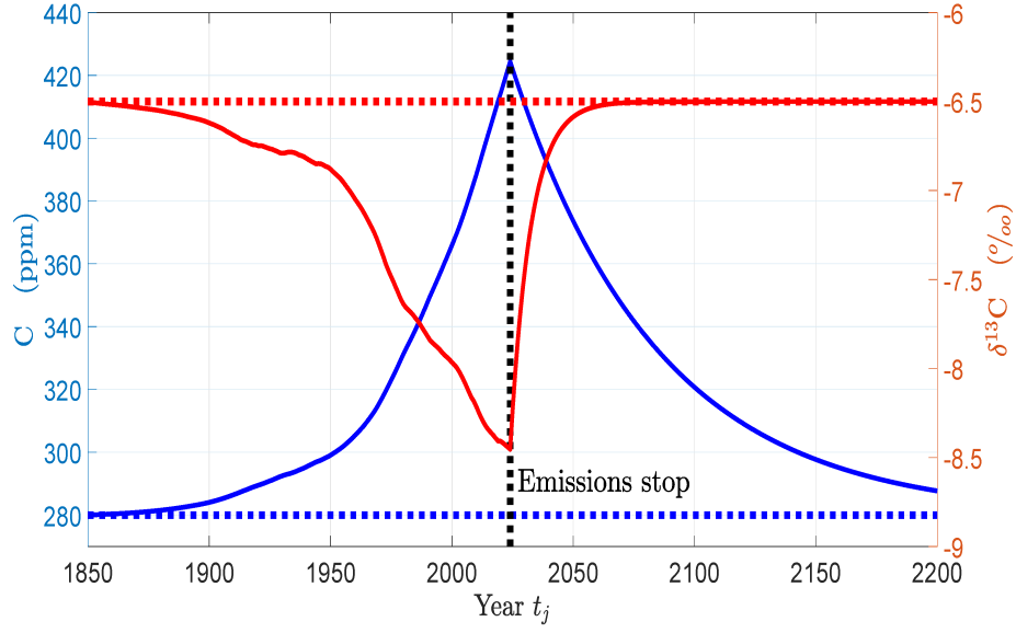
Figure 4: Modelled time dependence of atmospheric \text{CO}_2 concentration C and isotopic delta value \delta^{13}\text{C} if all fossil fuel emissions stopped after the year 2024, marked by the black dotted line. Because of isotope exchange, \delta^{13}\text{C} , shown as the smooth red line, evolves more quickly to its preindustrial value \delta^{13}\text{C}_0 = -6.5\text{‰} , shown as the red dotted line, than does the atmospheric concentration C , shown as the smooth blue line, to its preindustrial value, C_0 = 280 ppm, shown as the blue dotted line.
