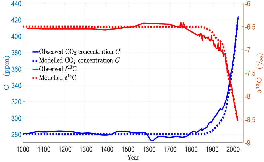
Figure 2: The continuous blue line shows observed yearly averages of \text{CO}_2 concentrations C = N/N_{\text{at}} in ppm (parts per million by volume) obtained from references [4, 5, 6, 7]. The continuous red line is observed isotope delta values \delta^{13}\text{C} found from references [8, 9, 10]. The corresponding dotted lines are model predictions from (73) and (74). The preindustrial concentrations of \text{CO}_2 were close to C_0 = 280 ppm and the preindustrial isotope delta values were close to \delta^{13}\text{C}_0 = -6.5 ‰. The e-folding time constant \tau_1 = 1/\gamma_1 of (73) for the decay of concentration perturbations, C - C_0 , was \tau_1 = 60 y. The e-folding time constant \tau_2 = 1/\gamma_2 of (74) for the decay of perturbations, C \times \delta^{13}\text{C} - C_0 \times \delta^{13}\text{C}_0 , of concentration-delta-value products was \tau_2 = 8 y.
