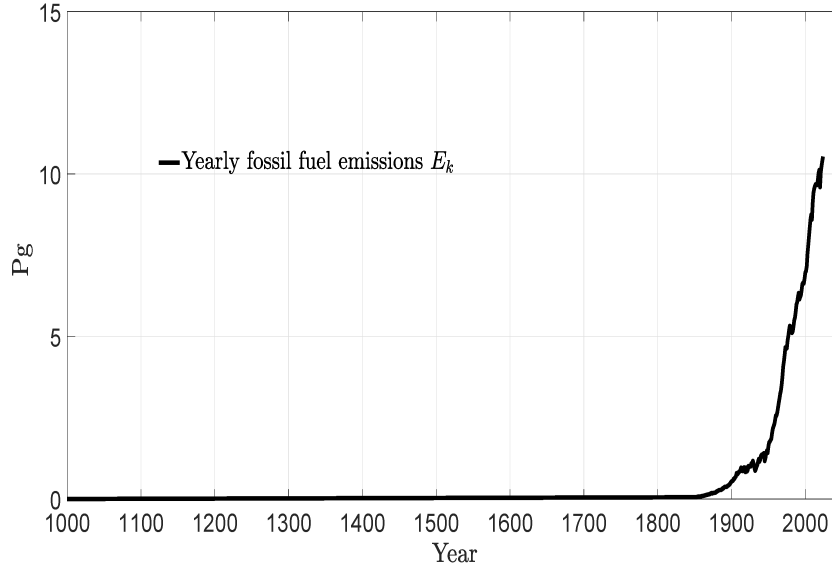
Figure 1: Yearly fossil fuel emissions of \text{CO}_2 to the atmosphere in petagrams (Pg) or 10^{15} g calendar year. The observational data is from reference [2, 3].
