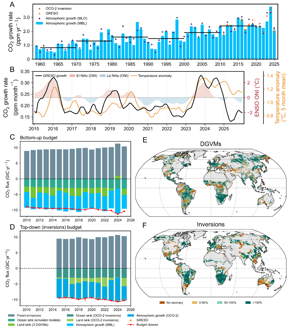
Fig. 1 Atmospheric CO 2 growth rate from 1959-2025, global carbon budget from 2010-2025 and spatial recovery of the 2023-2024 land sink losses in 2025. (a) Annual atmospheric CO 2 growth rates from globally averaged marine boundary layer observations (MBL, blue bars), the Mauna Loa station (MLO, dark blue squares), OCO-2 constrained atmospheric inversions (brown squares), and the Growth Rates Using Satellite Observations approach (GRESO, orange squares). GRESO values are based on GOSAT for 2010–2014 and on the mean of independently derived OCO-2 and GOSAT estimates from 2015 onward. (b) Monthly GRESO CO 2 growth rate (black line), Oceanic Niño Index (ONI; red and blue shading for El Niño and La Niña conditions, respectively), and global surface temperature anomaly (orange line, 5-month running mean) from 2015 to 2025. (c) Global bottom-up
