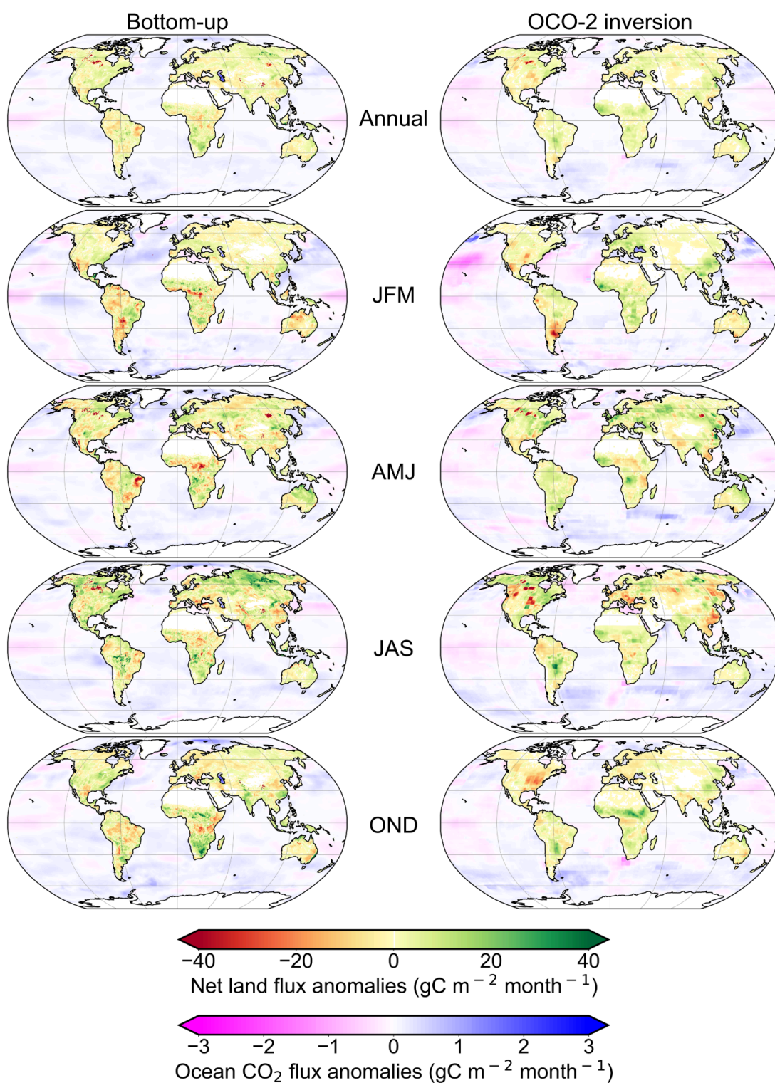
Fig. S1 Net land and ocean \text{CO}_2 flux anomalies for each quarter in 2025 compared with the 2015-2022 average for bottom-up models (left column) and the OCO-2 inversions (right column). Positive values represent increased flux from the atmosphere to the land or ocean (carbon sink).
