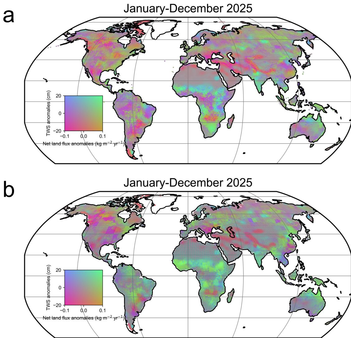
Fig. S2 Bivariate plots showing co-variations between net land flux anomalies from (a) DGVMs and (b) inversions and total water storage anomalies from the GRACE satellites in 2025. Green areas show wetter anomalies coincident with more CO 2 uptake, and magenta areas show drier anomalies that are coincident with reduced CO 2 uptake.
