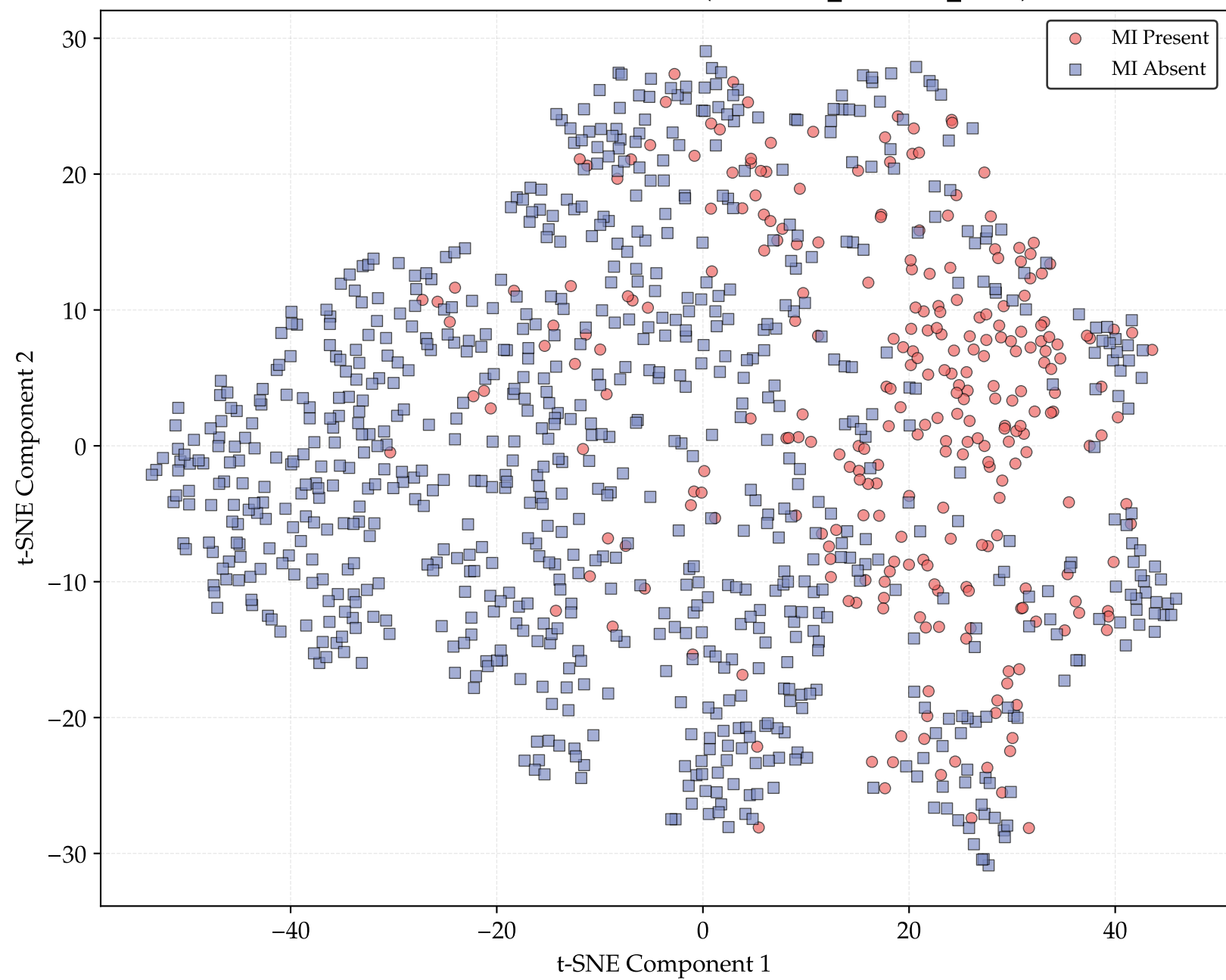
t-SNE Visualization - MI Class (HYBRID_SERIAL_REV)
