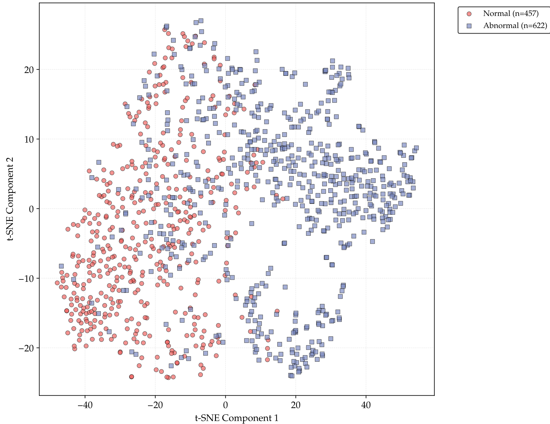
t-SNE Visualization (HYBRID_PARALLEL)
