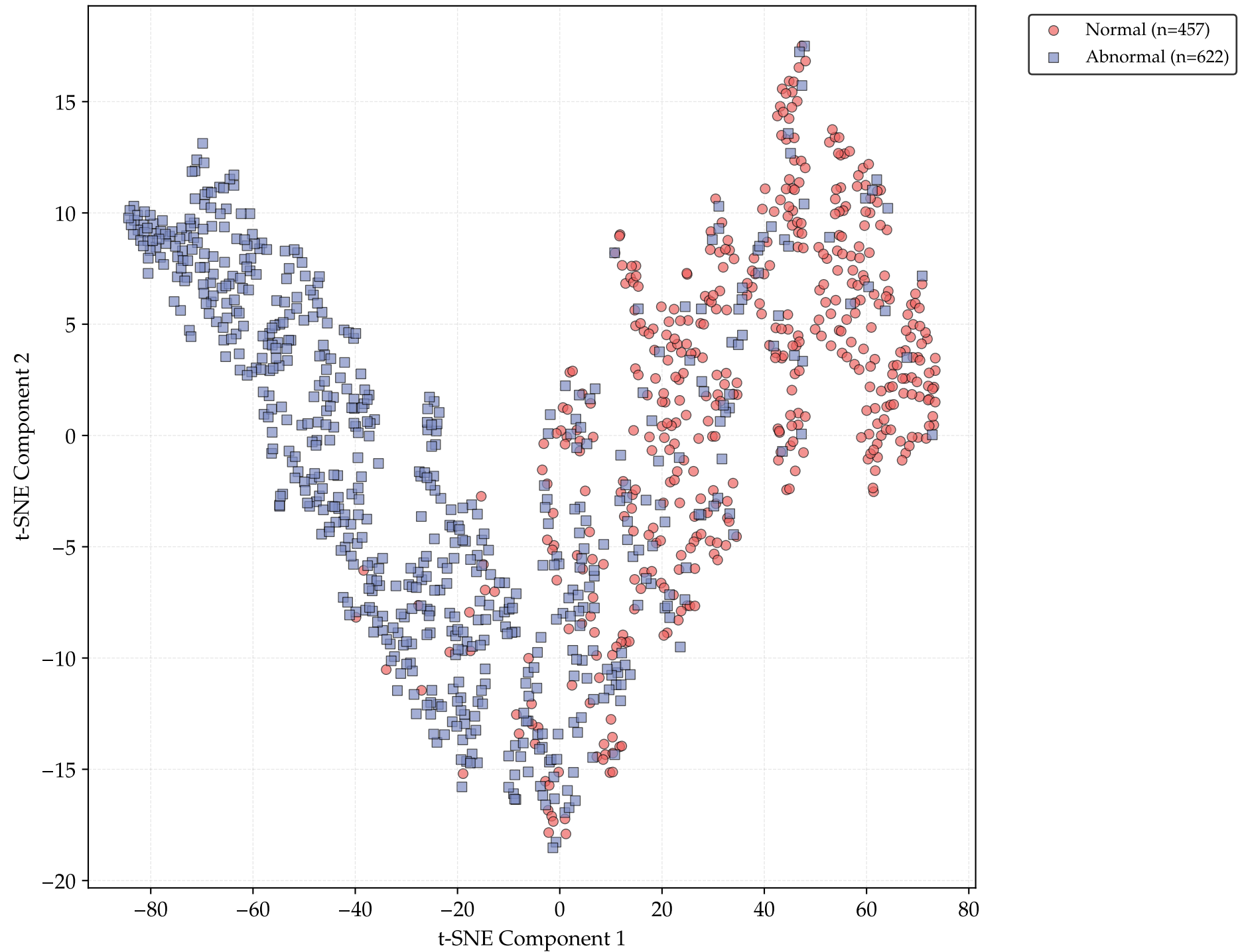
t-SNE Visualization (HYBRID_SERIAL_REV)
