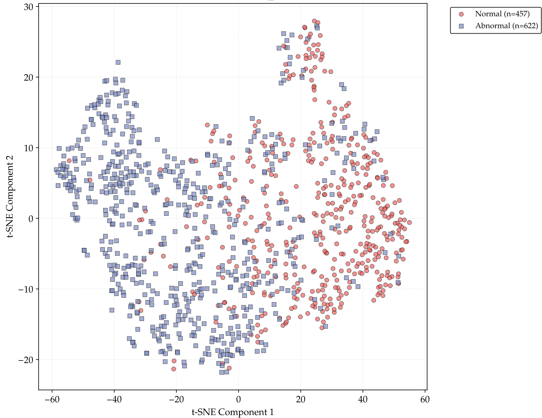
t-SNE Visualization (HYBRID_CROSSATTN)
