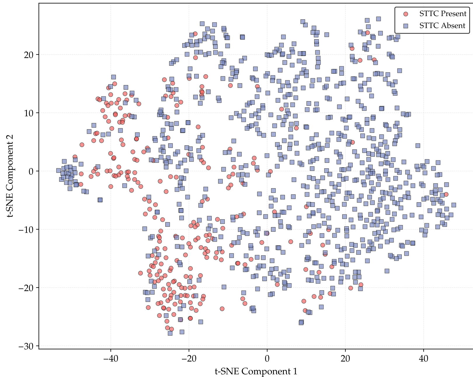
t-SNE Visualization - STTC Class (HYBRID_CROSSATTN)
