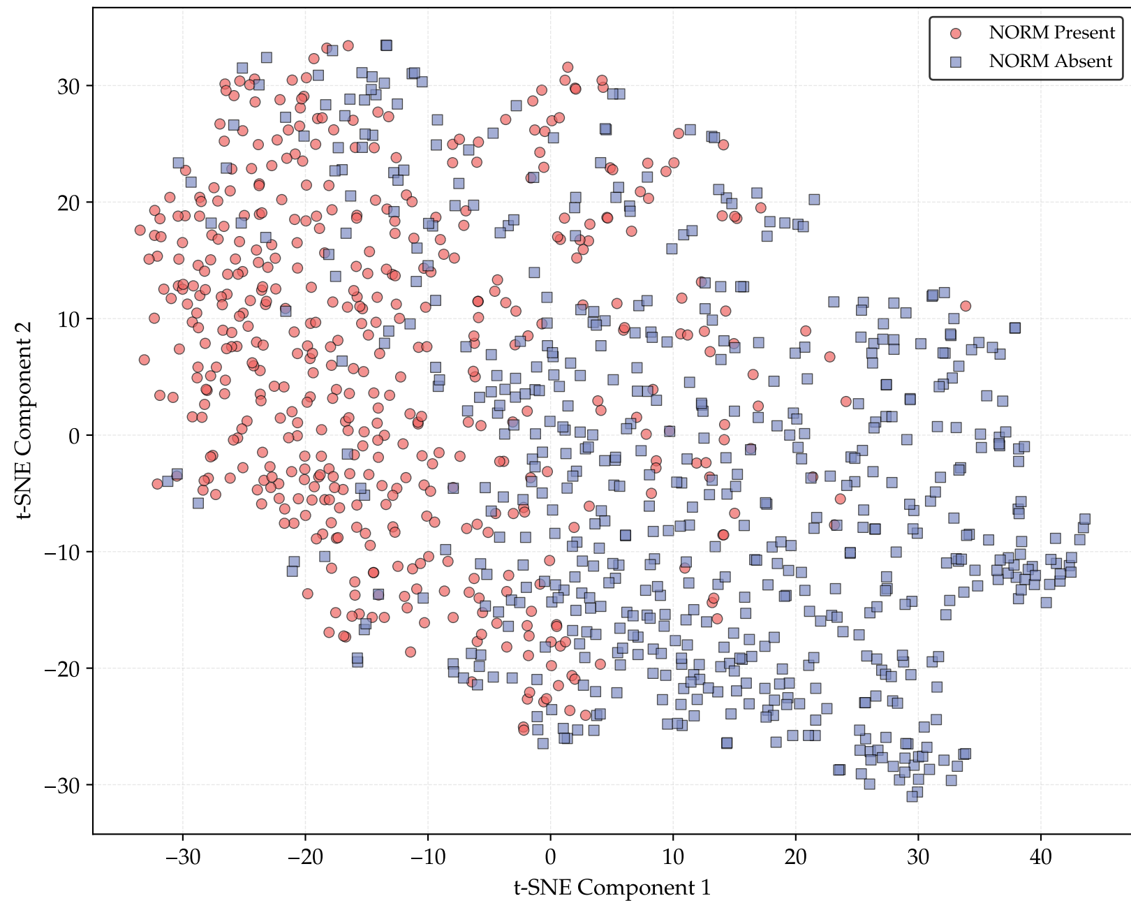
t-SNE Visualization - NORM Class (HYBRID_PARALLEL)
