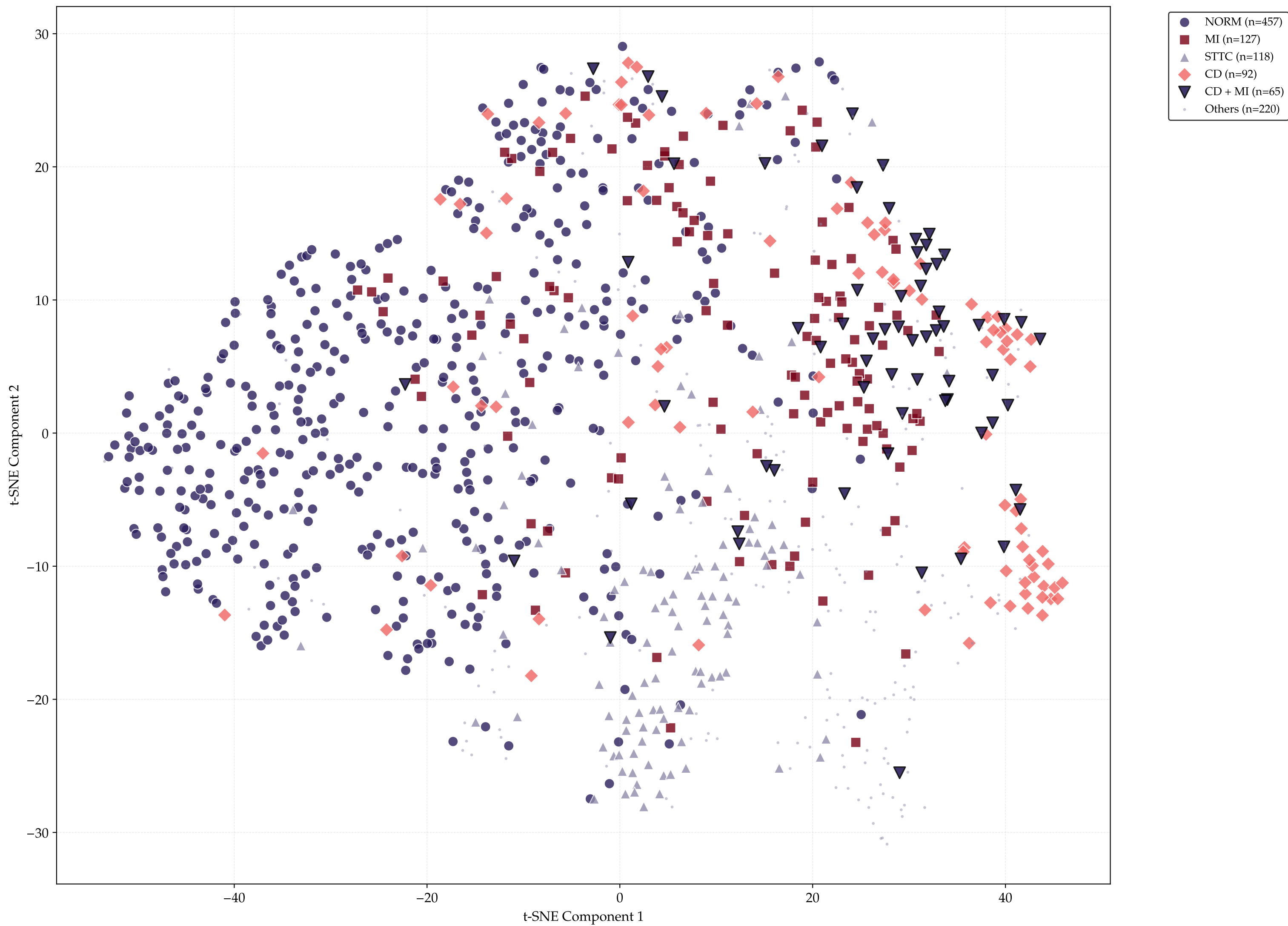
Multilabel t-SNE Overview - Major Label Combinations (HYBRID_SERIAL_REV)
