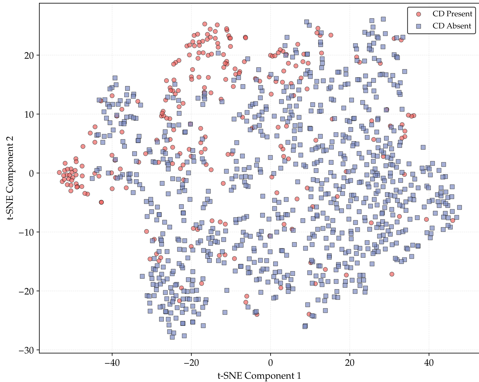
t-SNE Visualization - CD Class (HYBRID_CROSSATTN)
