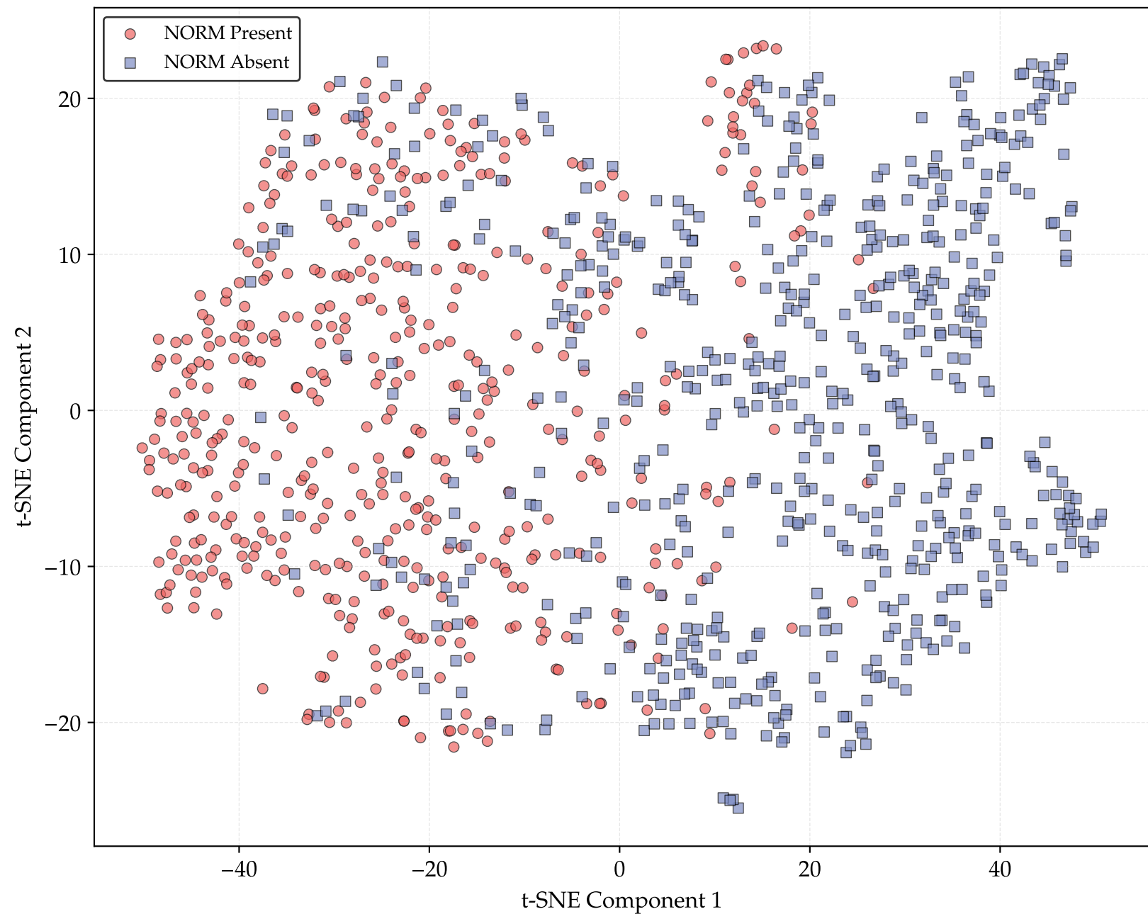
t-SNE Visualization - NORM Class (HYBRID_SERIAL_REV)
