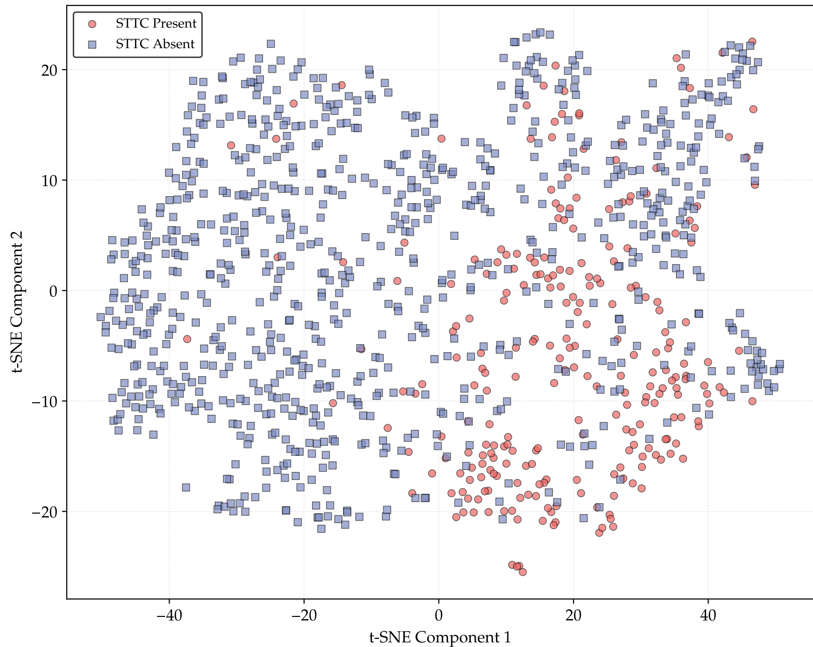
t-SNE Visualization - STTC Class (HYBRID_SERIAL_REV)
